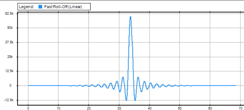
Linear phase fast roll-off filter
