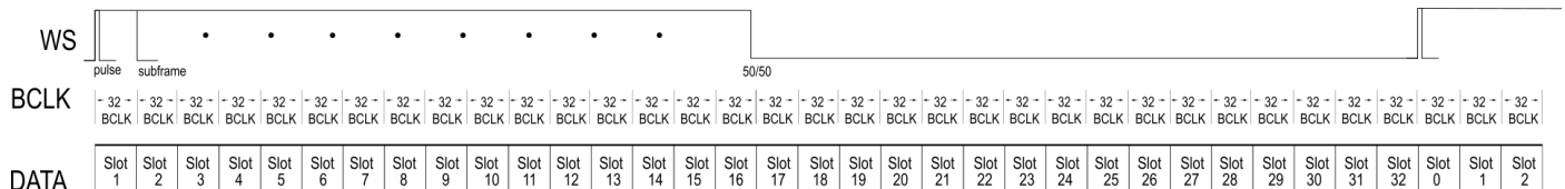
Figure 9 – TDM1024 mode
