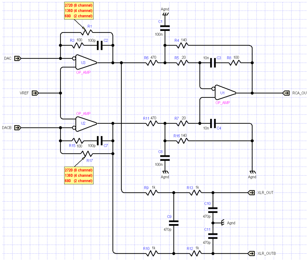
Figure 7 - Recommended Differential, Current-Mode External Op-Amp Circuit
