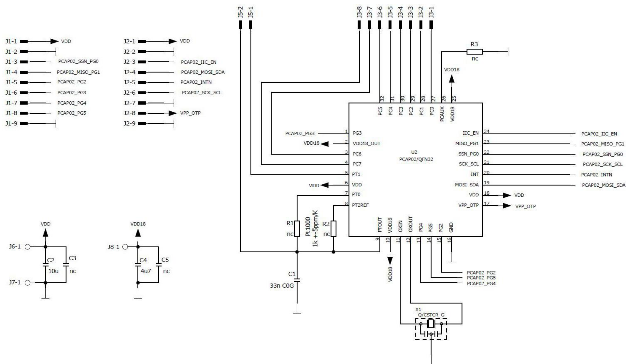
Figure 4-2: PCaO 2 AD module schematics
