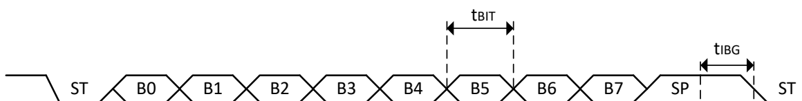
Figure 2-1 UART timing
