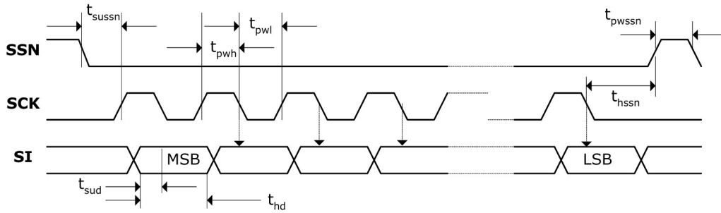
Figure 2-1: SPI Write
