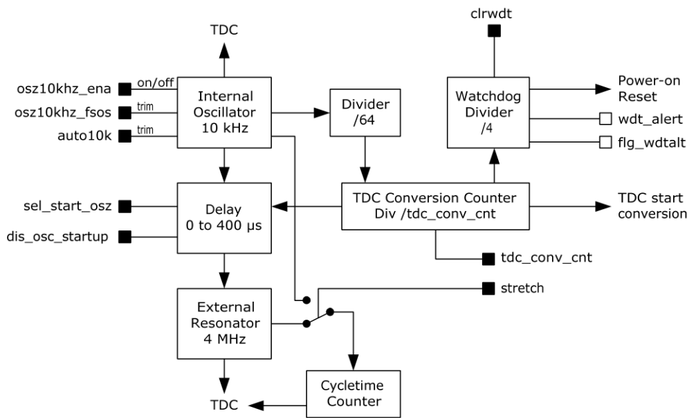
Figure 3-1: Clock Generation
