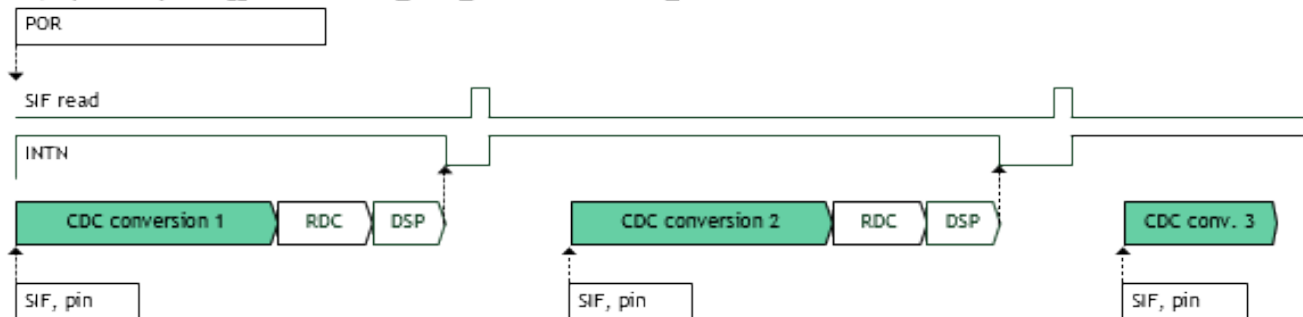
Figure 13: Conversion Modes
