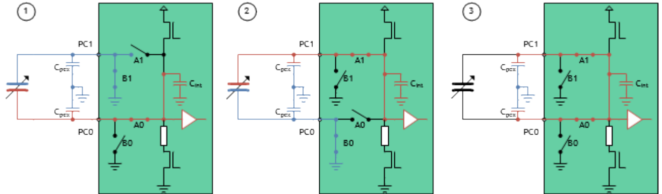
Figure 16: External Compensation
