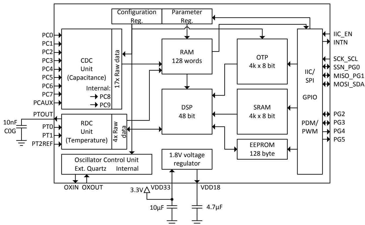
Figure 1-1 Blockdiagram
