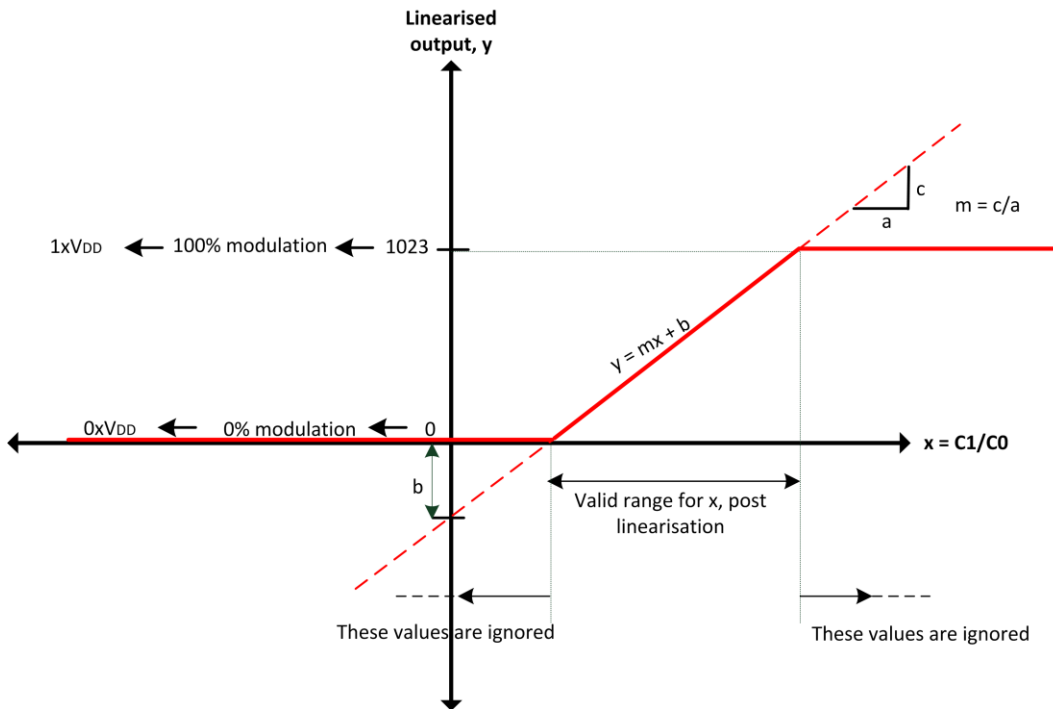
Figure 4-8: PWM-PDM linearization
