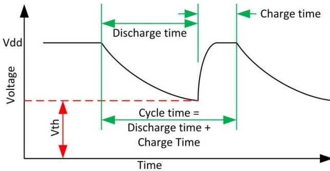
Figure 3-1 Cycle Time
