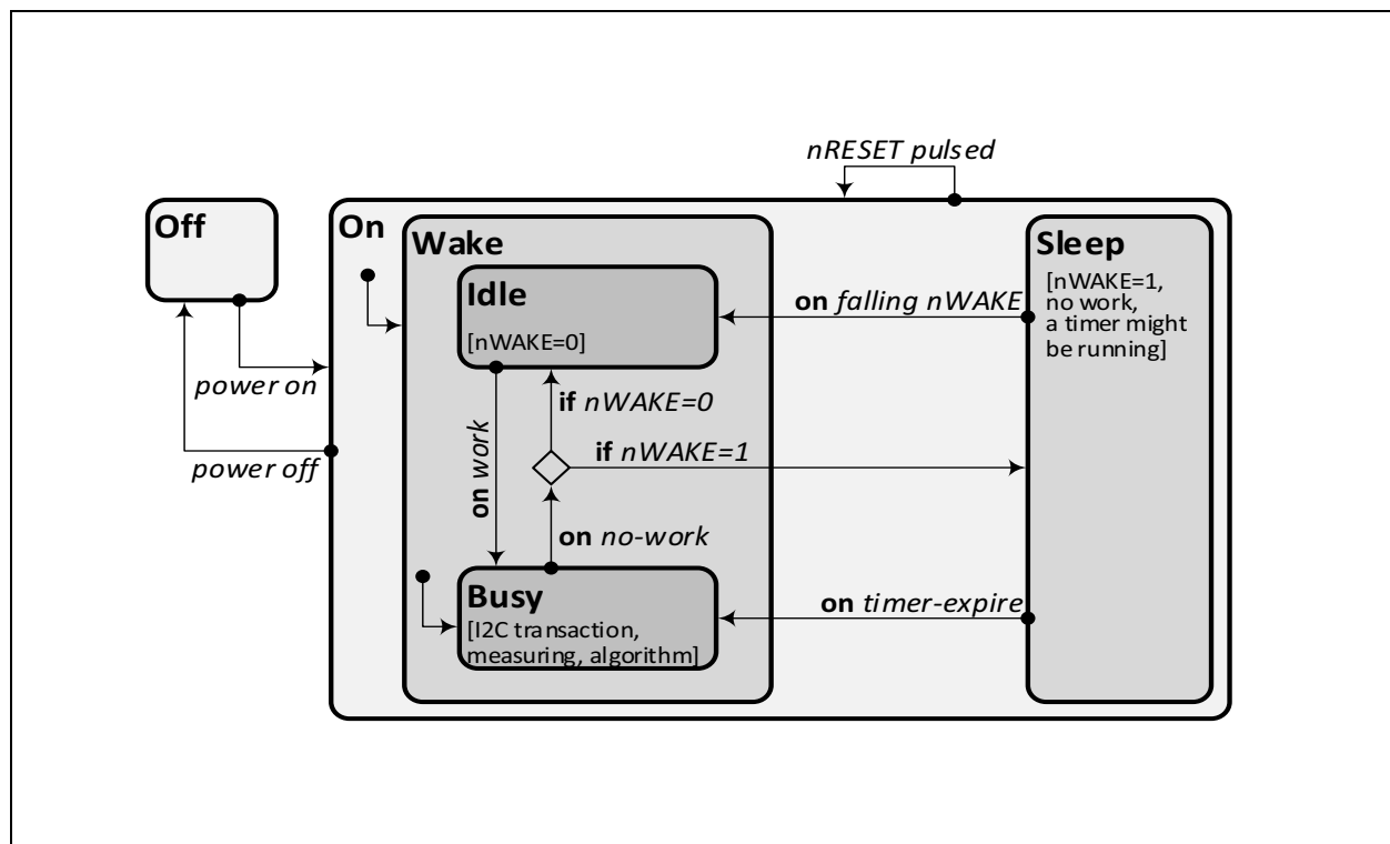
Figure 10: CCS811 Power States
