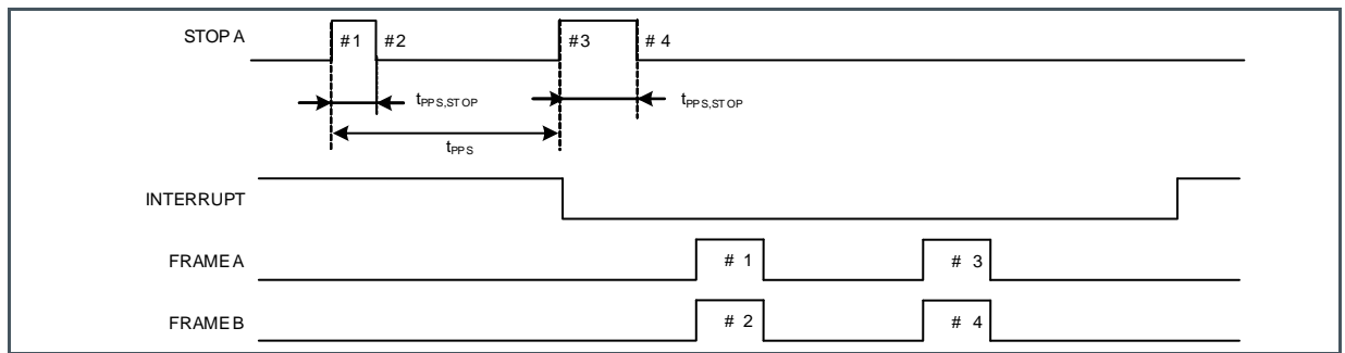
Figure 39: Channel Combination Pulse Width Measurement
