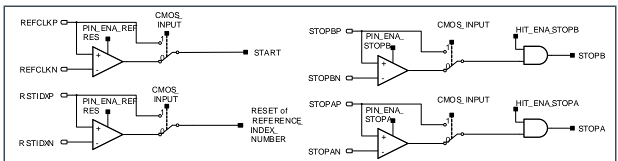
Figure 40: Input Circuitry
