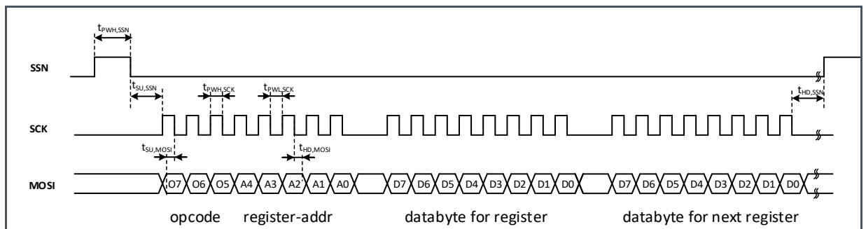
Figure 15: Write and Incremental Write
