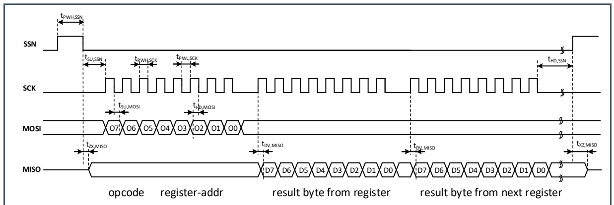
Figure 16: Read and Incremental Read
