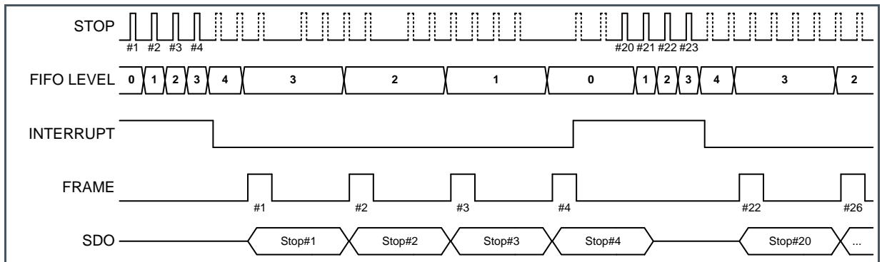
Figure 64: BLOCKWISE_FIFO_READ
