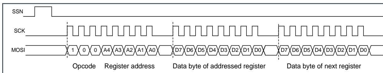
Figure 53: SPI Incremental Write
