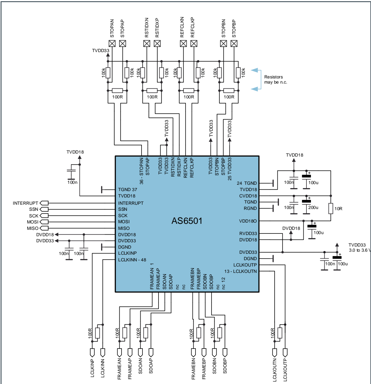
Figure 3: AS6501 QFP48
