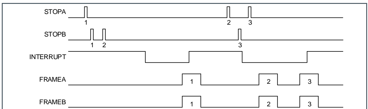
Figure 65: COMMON_FIFO_READ
