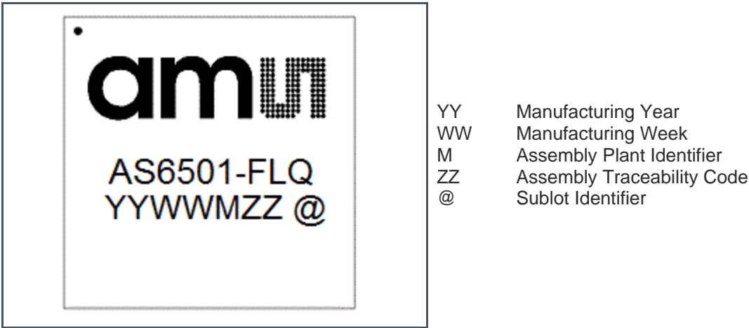
Figure 68: QFP48 Package Marking/Code
