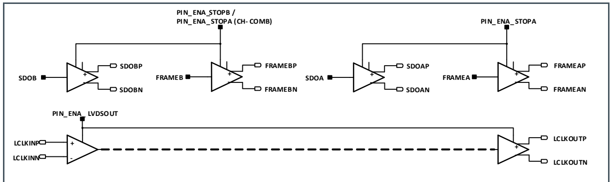
Figure 46: LVDS Outputs
