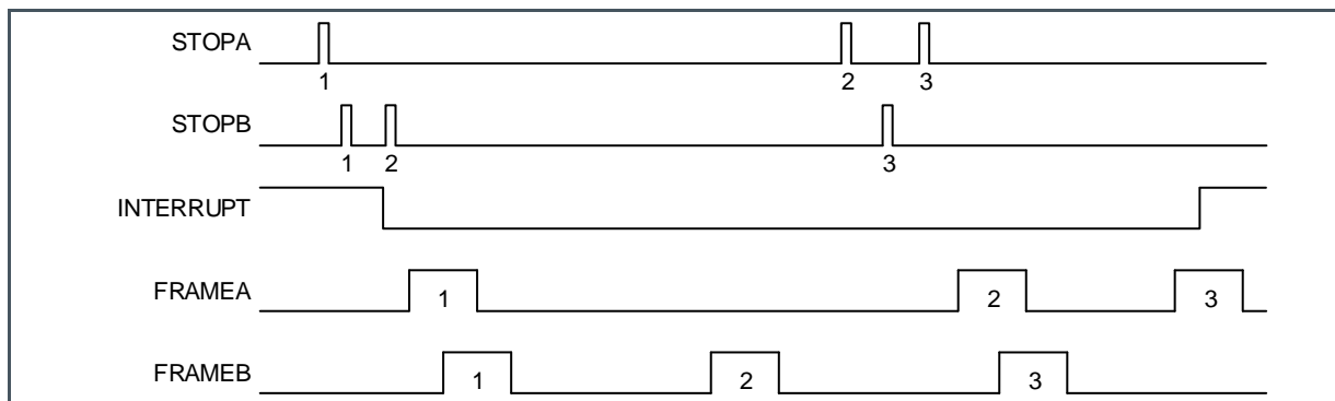
Figure 63: Stops On Both Channels
