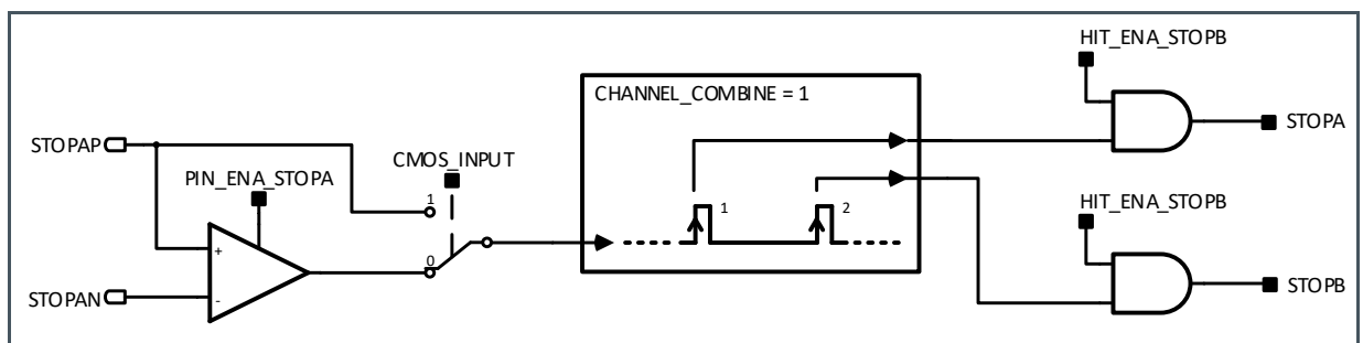
Figure 36: Channel Combination Low Pulse-to-Pulse Spacing
