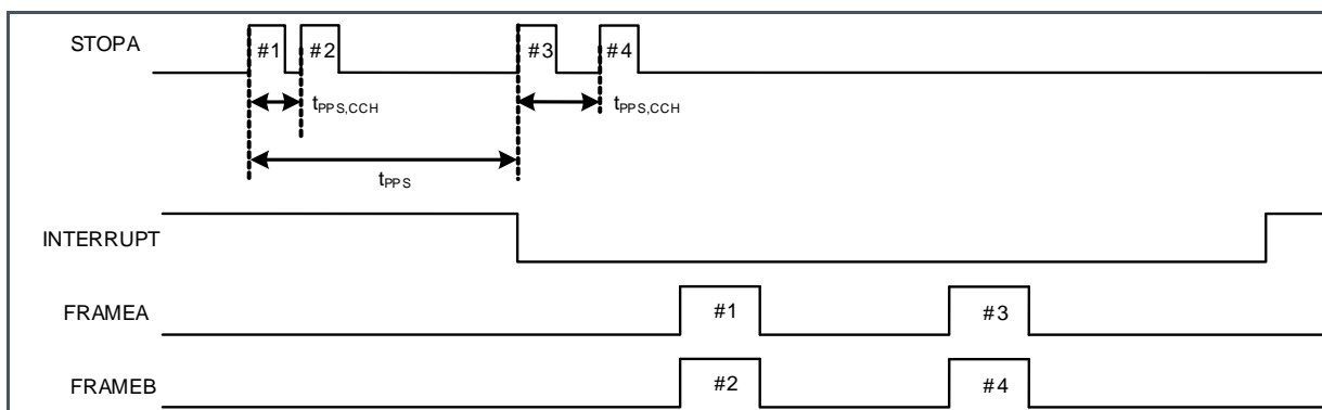
Figure 37: Channel Combination Low Pulse-to-Pulse Spacing
