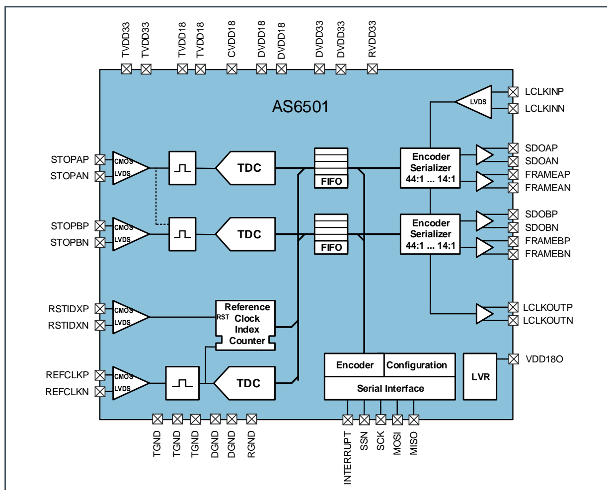
Figure 2: Functional Blocks of AS6501
