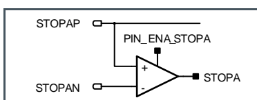
Figure 43: LVDS (CMOS_INPUT=0):
