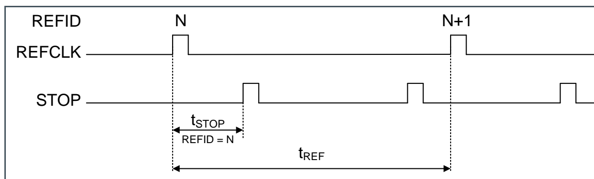
Figure 33: AS6501 Time Measurement
