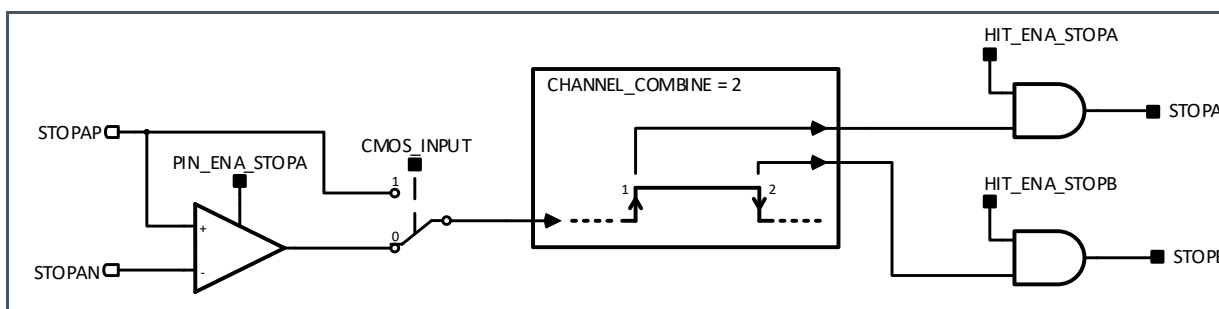
Figure 38: Channel Combination Pulse Width Measurement
