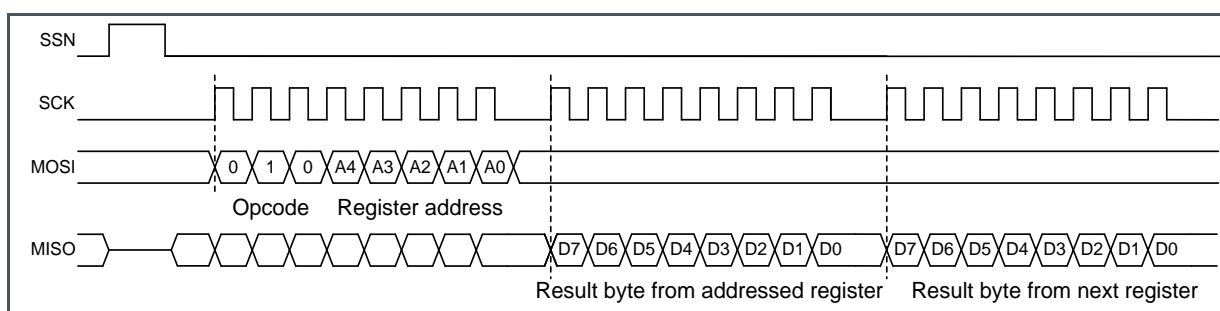
Figure 54: SPI Incremental Read
