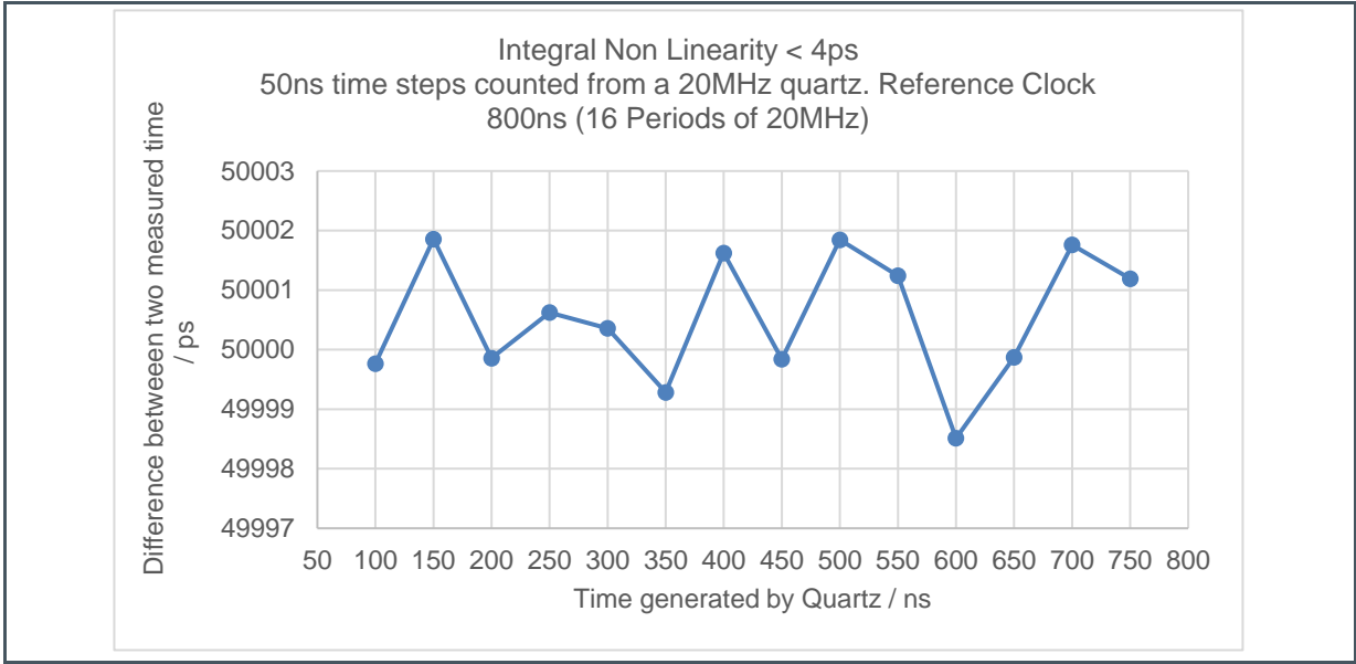
Figure 21: Integral Non-Linearity
