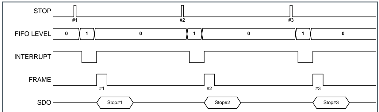
Figure 60: Input Stop Event Rate Is Lower than the Readout Rate
