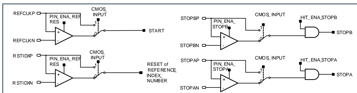
Figure 40: Input Circuitry
