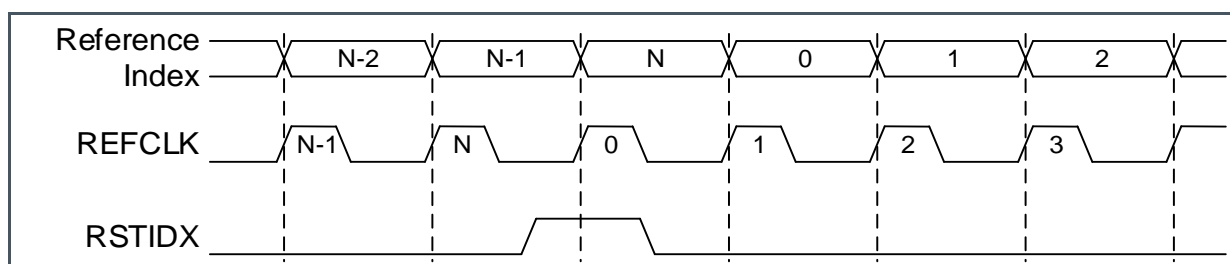
Figure 41: Reference Index Counter Reset
