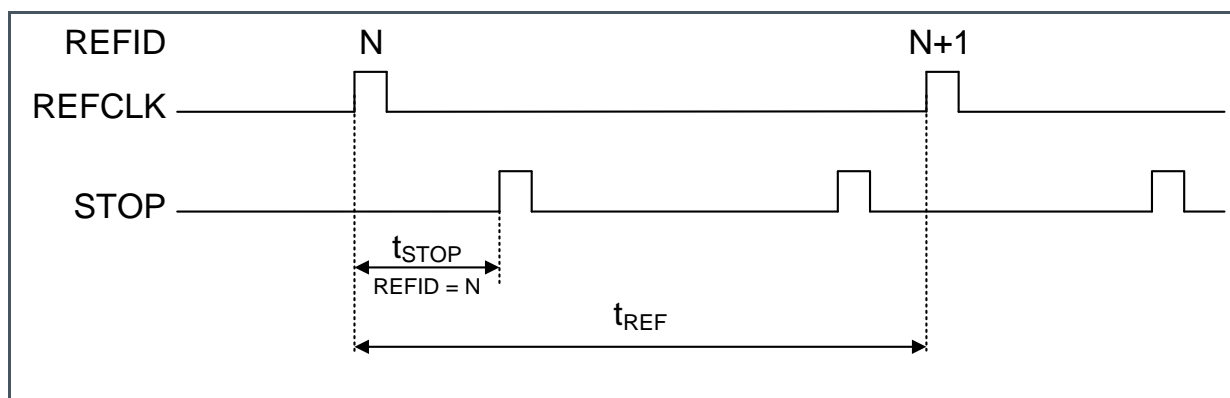
Figure 33: AS6501 Time Measurement
