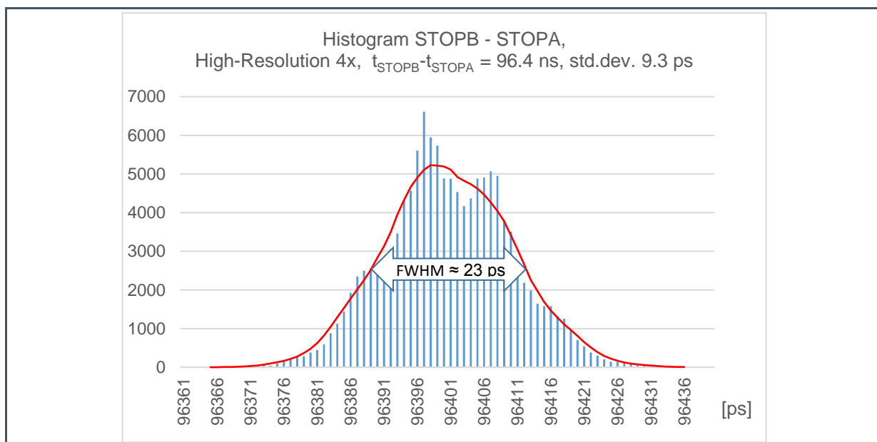
Figure 18: STOPB – STOPA, HIGHRES 4x, Histogram 100000 Values
