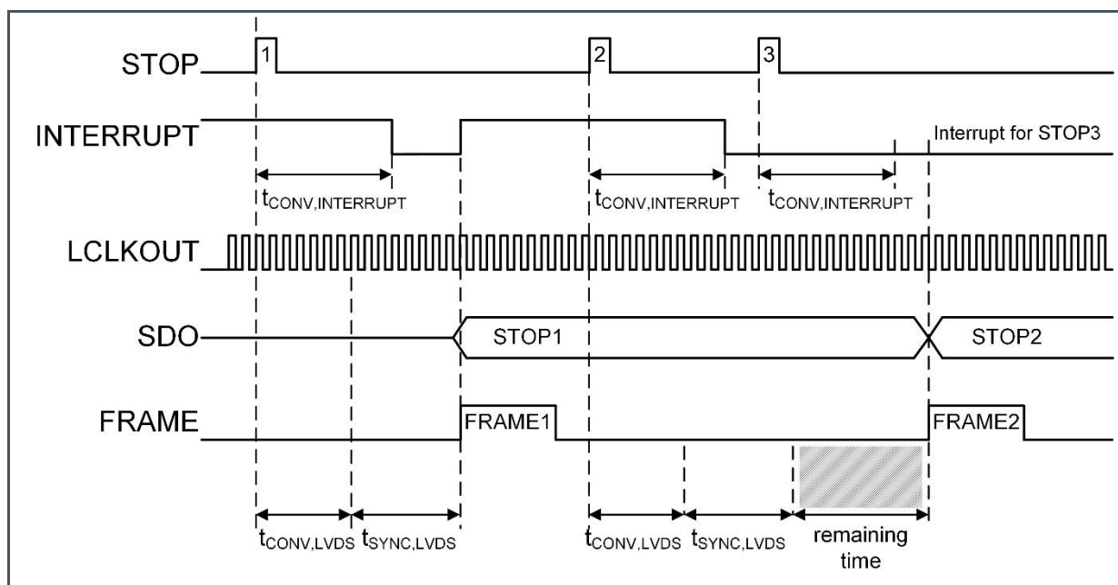
Figure 58: Conversion Latency
