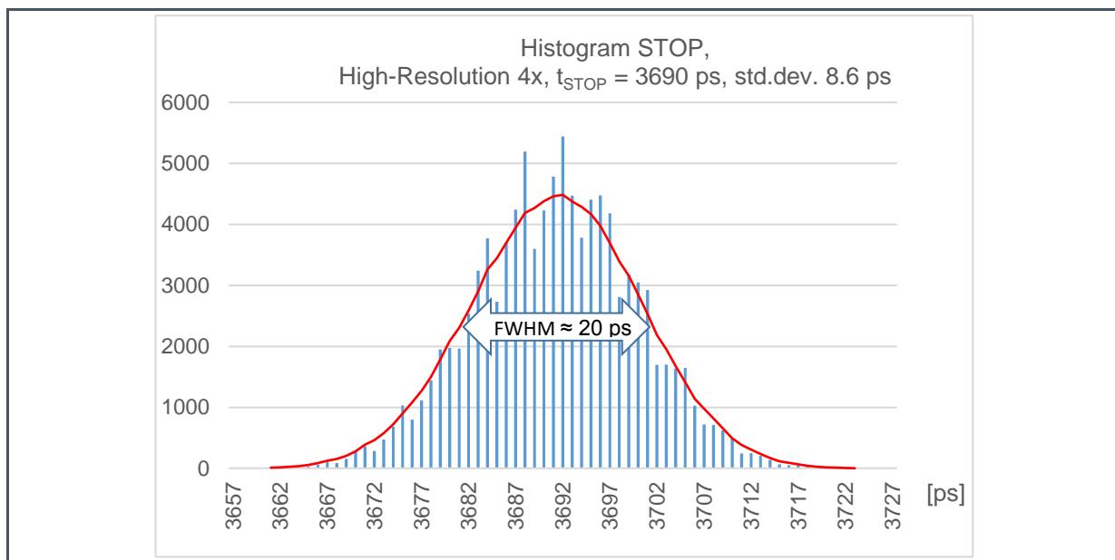
Figure 17: STOP, HIGHRES 4x, Histogram 100000 Values
