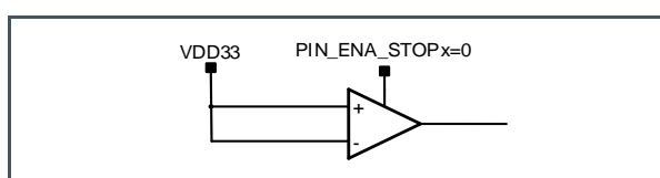
Figure 45: Unused LVDS
