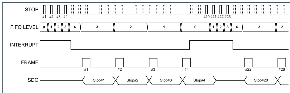
Figure 64: BLOCKWISE_FIFO_READ
