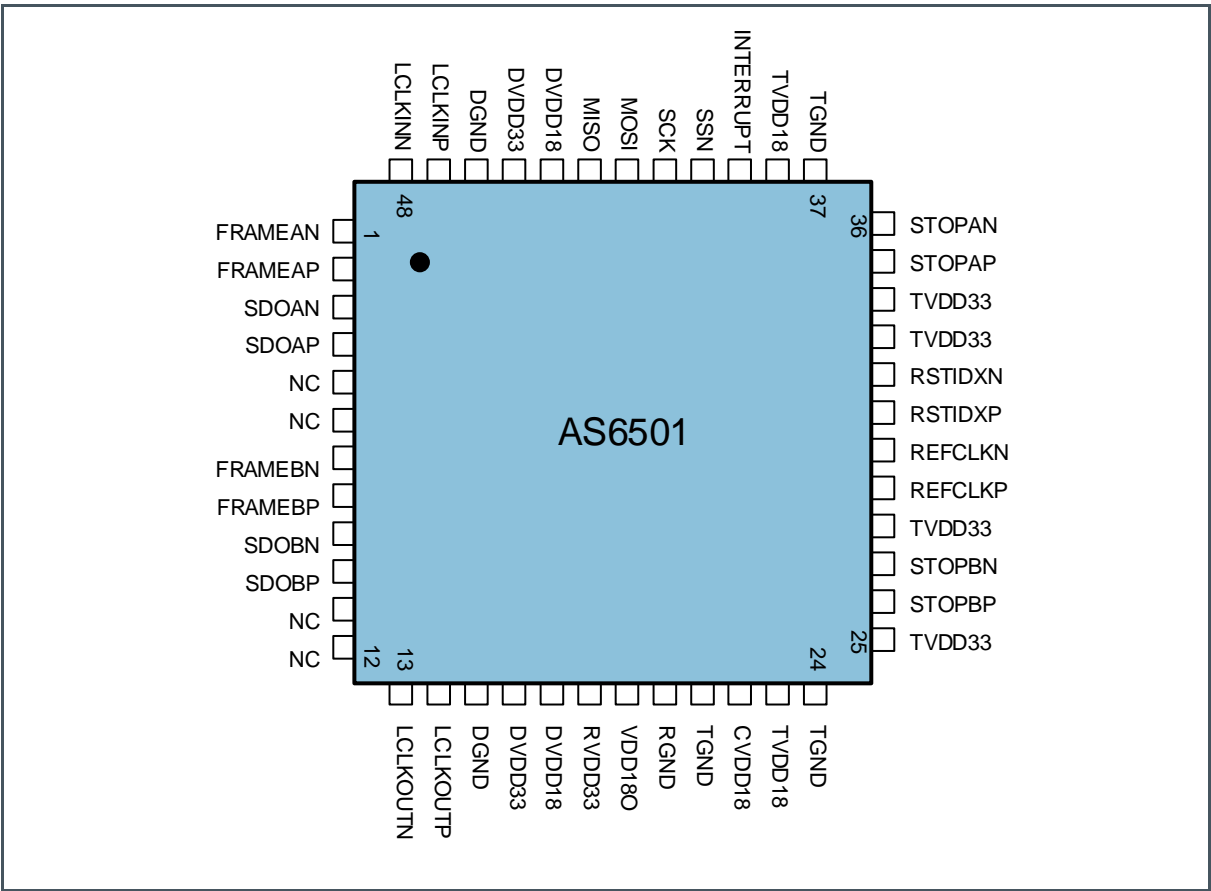
Figure 3: AS6501 QFP48
