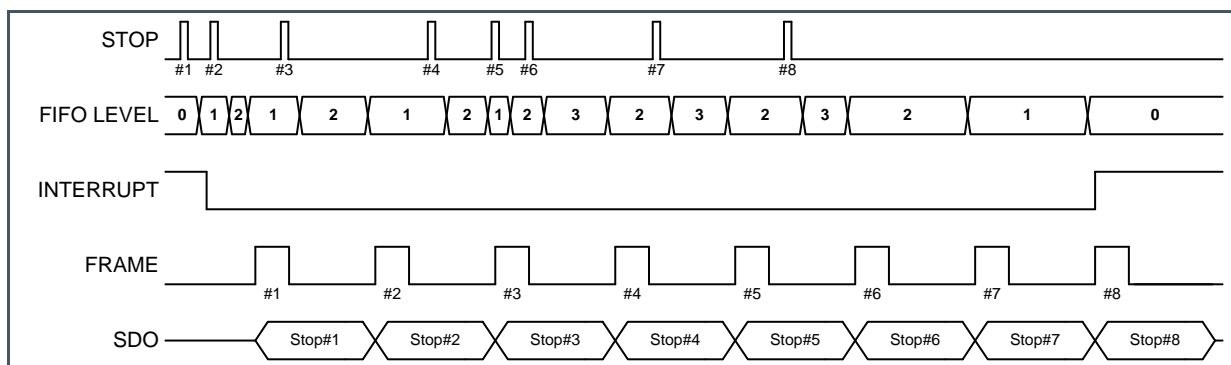
Figure 61: Average Stop Event Rate Is Lower, but Peak Stop Event Rate Is Higher than the Readout Rate
