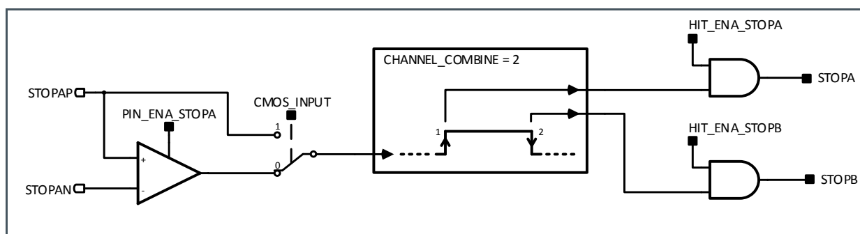
Figure 38: Channel Combination Pulse Width Measurement
