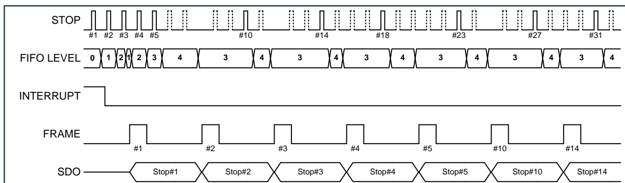
Figure 62: Stop Event Rate Is Higher than the Readout Rate
