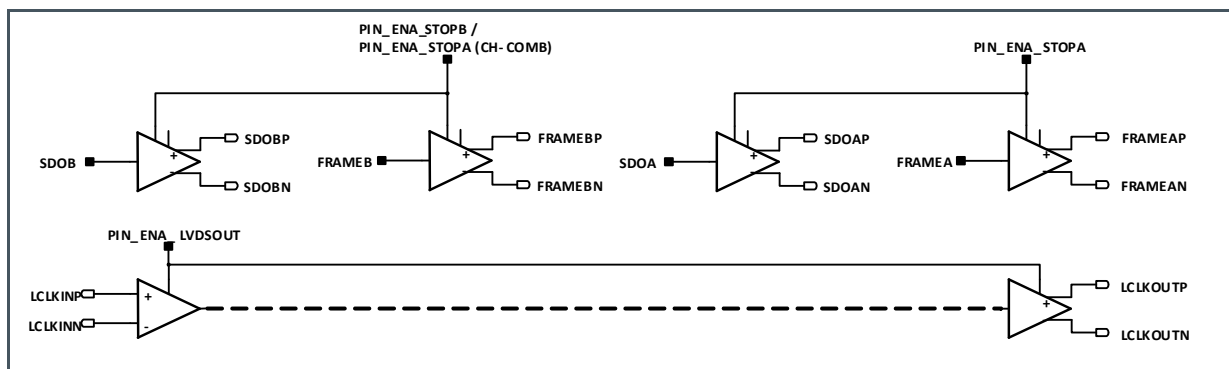
Figure 46: LVDS Outputs
