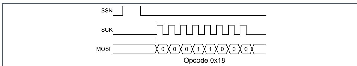
Figure 52: Init Reset Opcode
