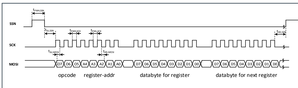
Figure 15: Write and Incremental Write
