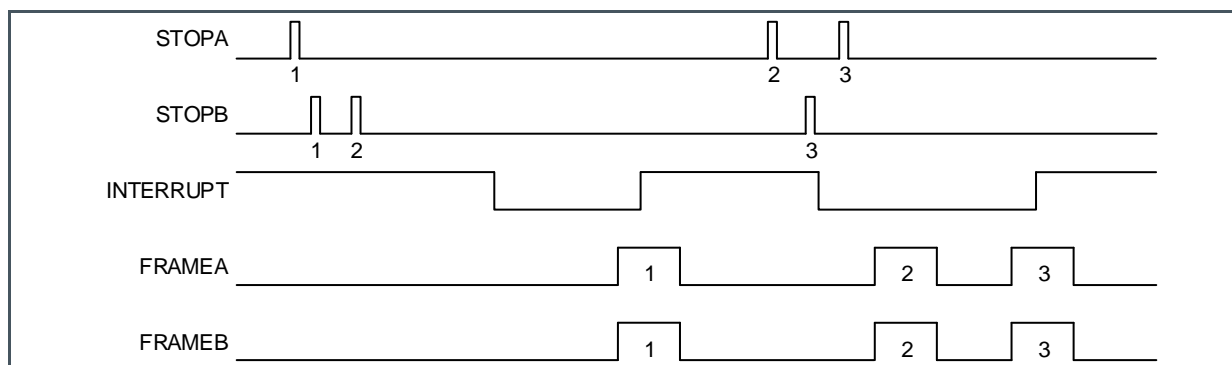
Figure 65: COMMON_FIFO_READ
