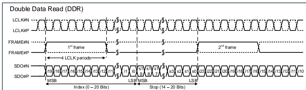
Figure 49: LVDS Outputs DDR
