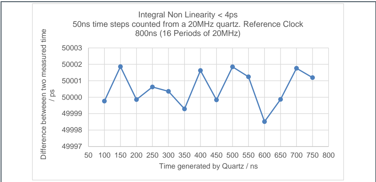
Figure 21: Integral Non-Linearity
