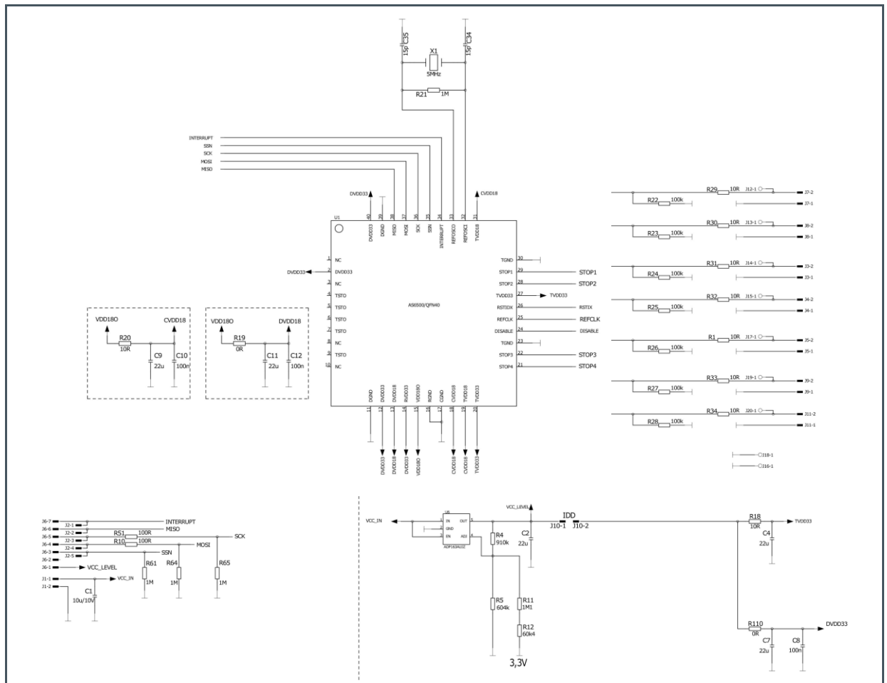
Figure 12: AS6500-QF_DK_RB Schematics
