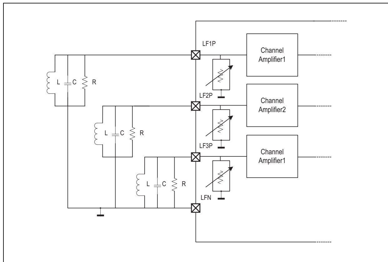
Figure 41: Antenna Dumper
