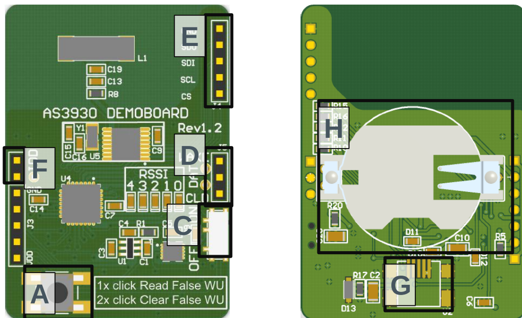
Figure 1: AS3930 Demoboard Description Top and Bottom
