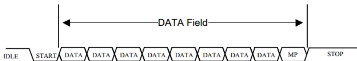
Figure 4: APC1 data byte structure
