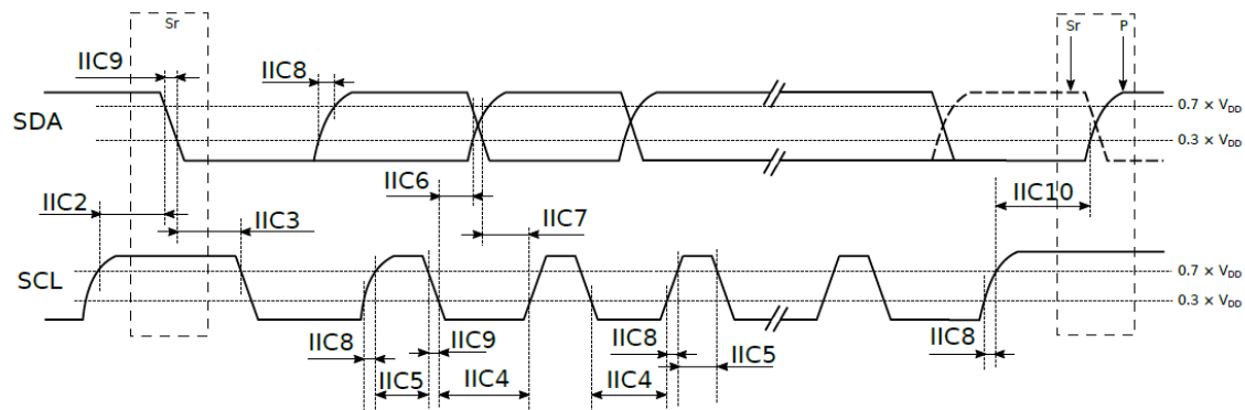
Figure 3-19 I2C Timing Diagram (HS mode)
