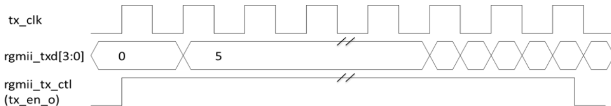
Figure 3-178 RGMII Transmit Waveform in 1000M
