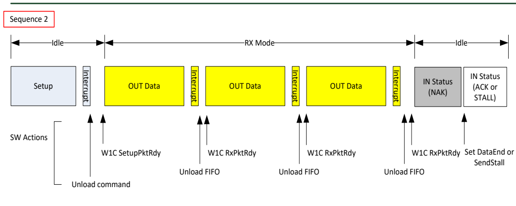
Figure 3-142 EP0 IDLE for RX Mode
