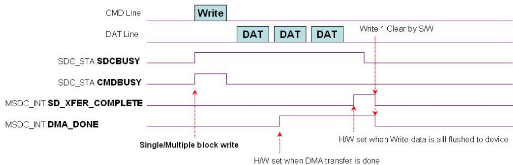
Figure 3-27 Single Block and Multi-block Write in DMA Mode
