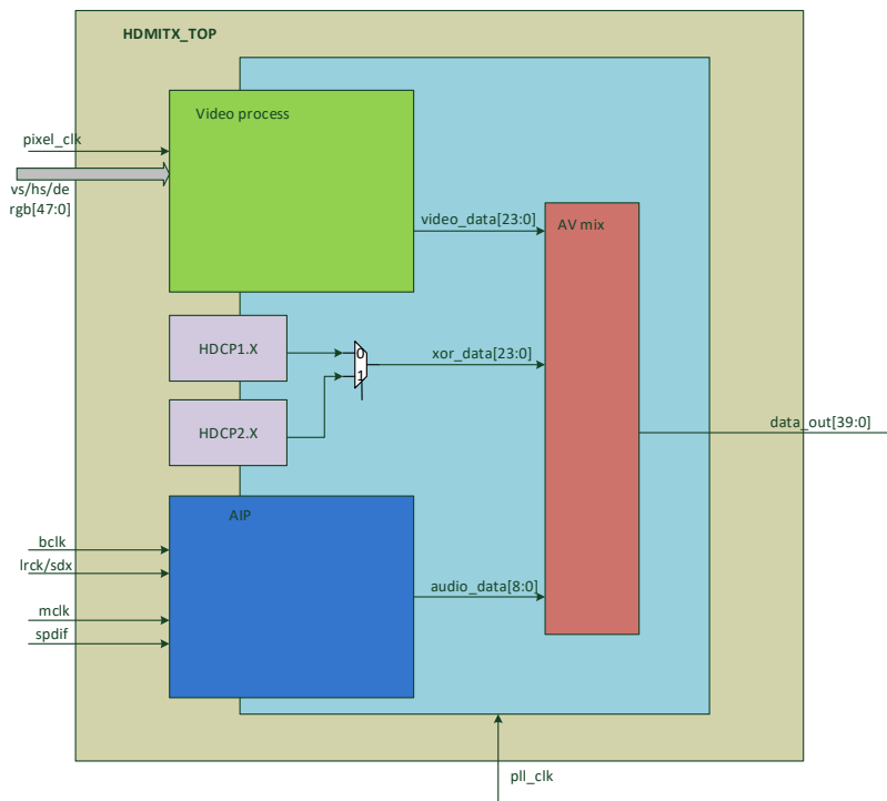
Figure 3-83 HDMITX Block Diagram
