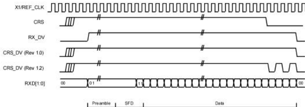
Figure 3-187 RMII Receive Waveform
