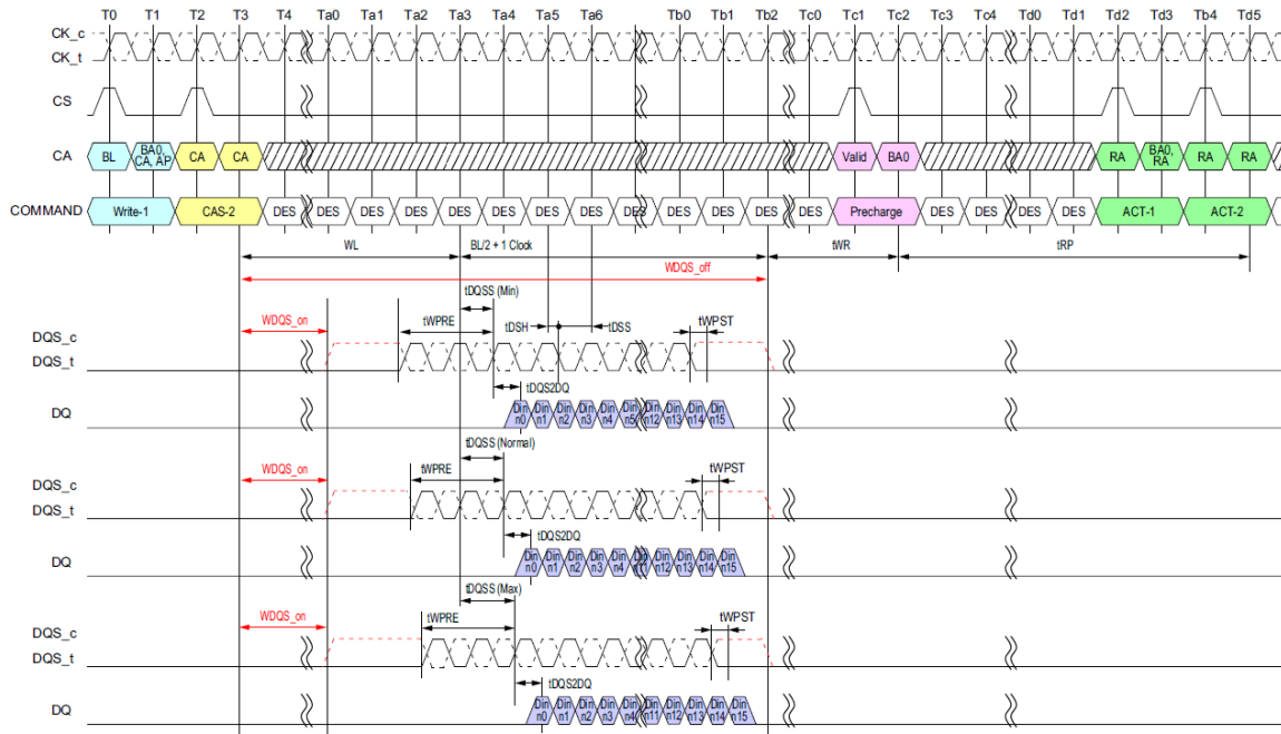
Figure 3-18 Write Operation
