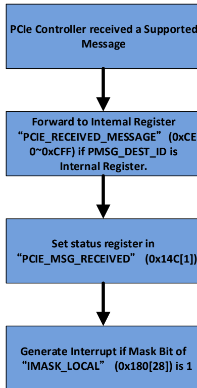
Figure 3-203 RC Received Other Supported Message Flow
