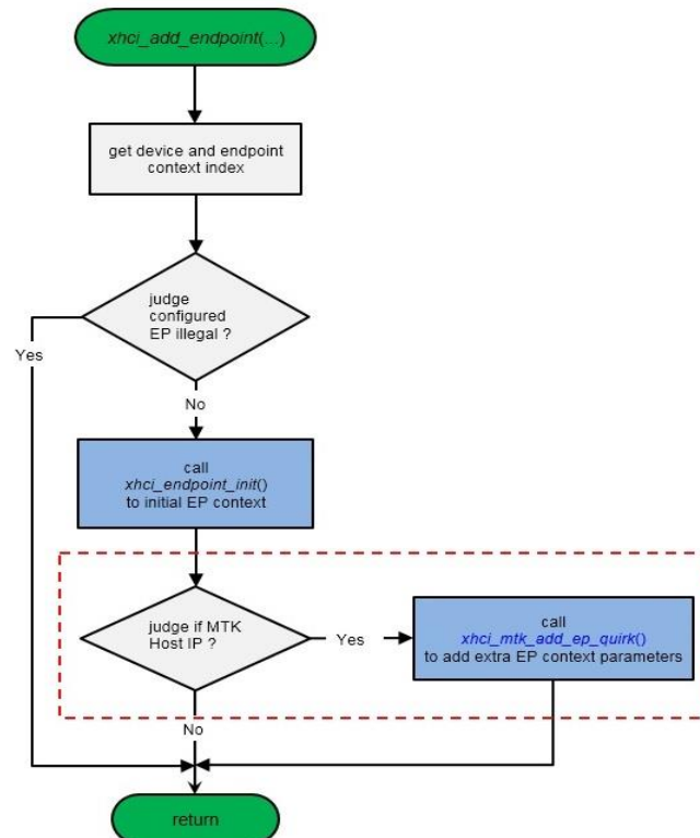
Figure 3-133 Patched xHCI_add_endpoint() Flow
