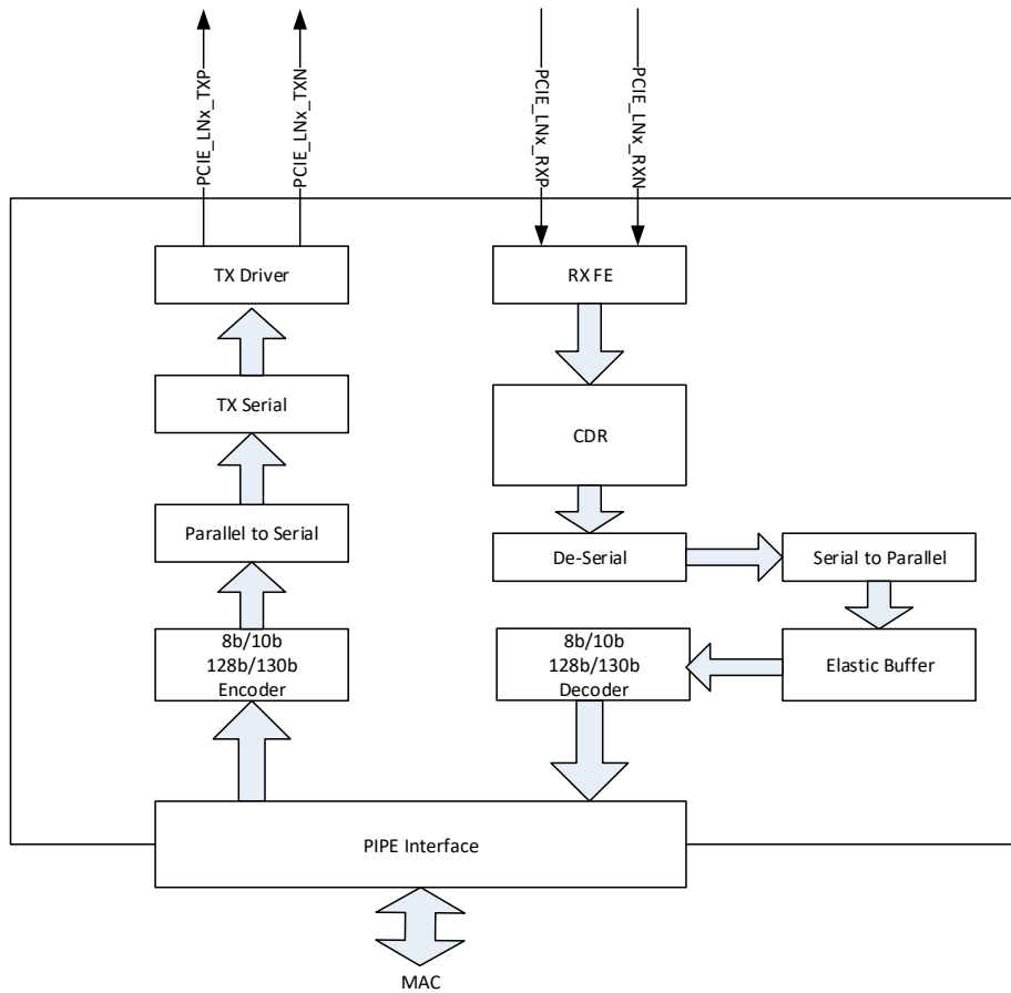
Figure 3-219 Block Diagram of PCIe PHY
