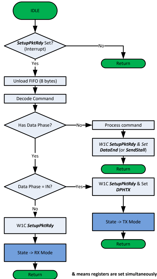
Figure 3-137 EP0 Idle Flow Chart
