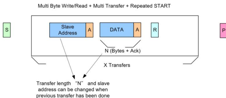
Figure 3-111 Repeated START Multiple Transfers (Write/Read Mode)
