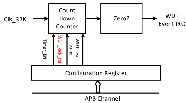
Figure 3-14 SCP WDT Block Diagram
