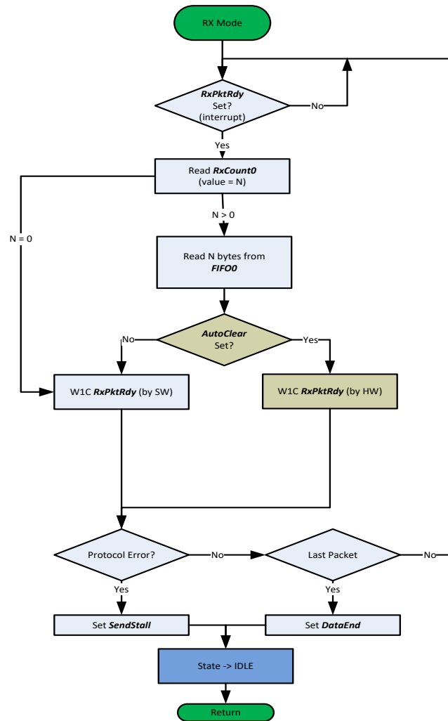
Figure 3-141 EP0 RX Mode Flow Chart
