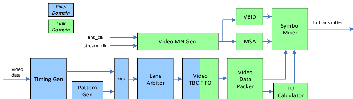
Figure 3-70 EDP TX Encoder Block Diagram
