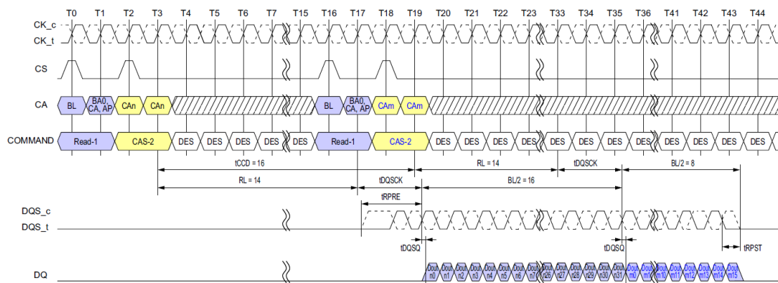
Figure 3-19 Read Operation
