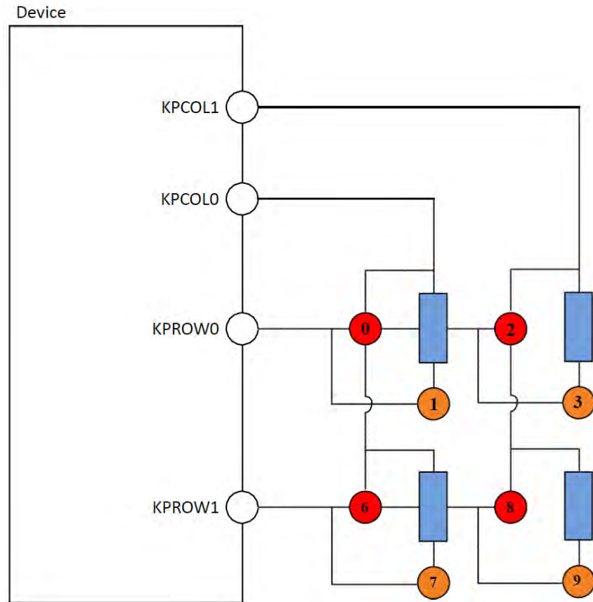
Figure 3-49 2 × 2 Keypad Matrix (8 Keys)
