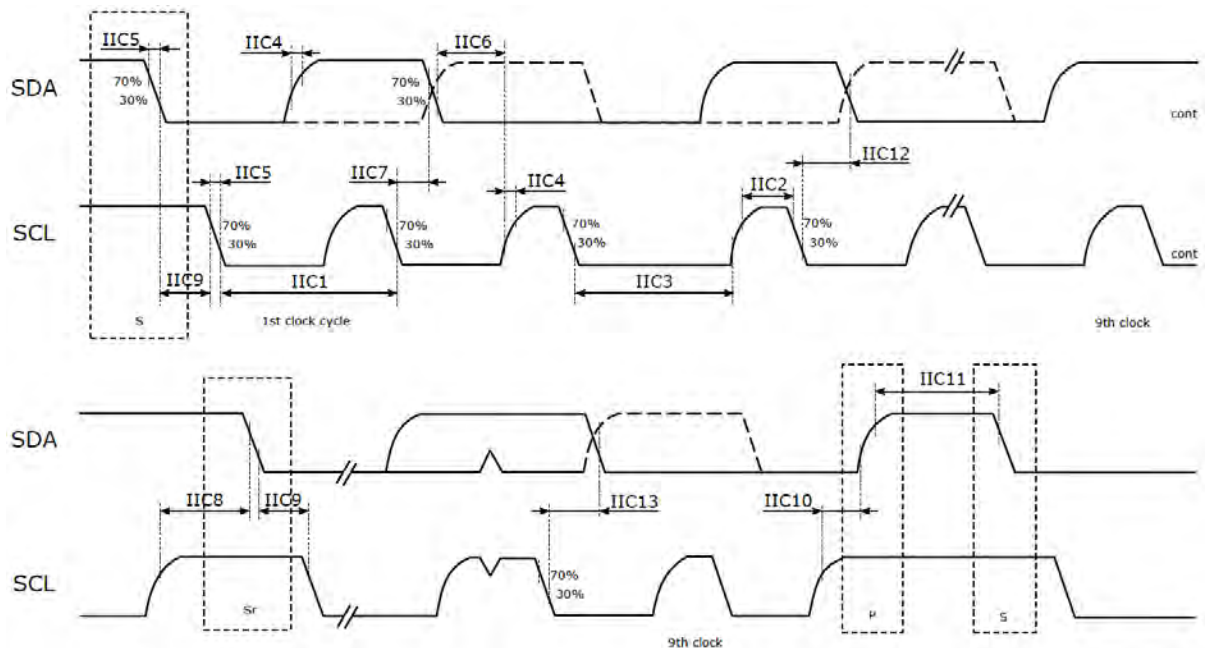
Figure 3-45 I2C Timing Diagram
