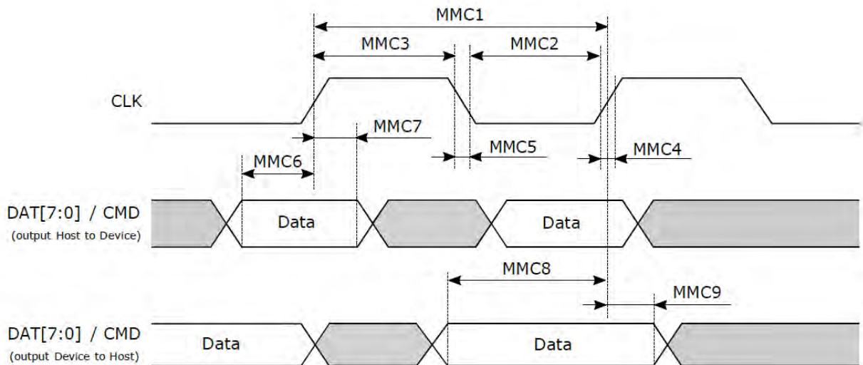
Figure 3-7 eMMC Timing Diagram (backward-compatible device interface)
