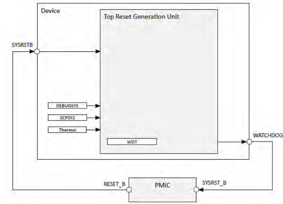
Figure 5-2 Reset Block Diagram
