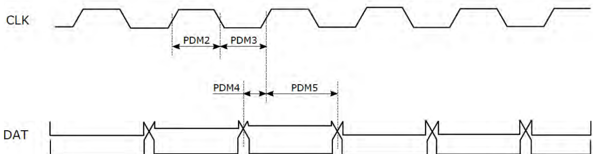
Figure 3-44 PDM Timing Diagram
