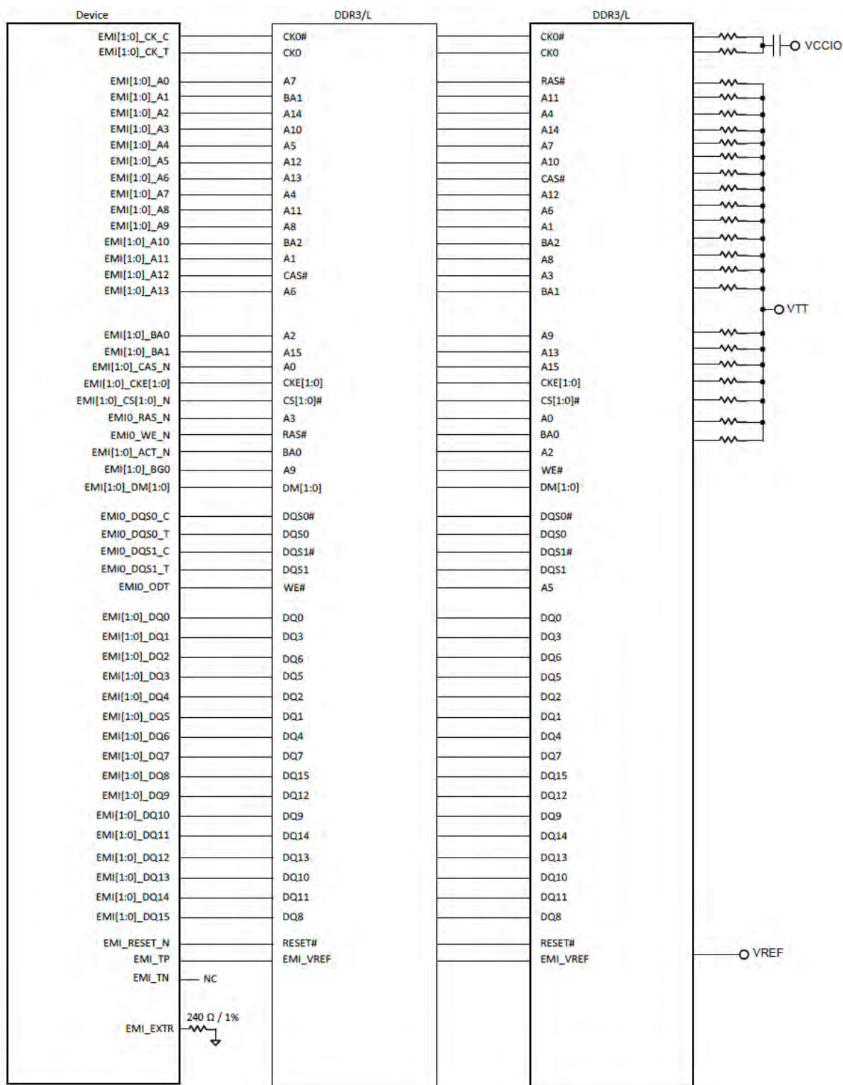
Figure 3-2 DDR3/L Basic Schematic for 2 x 16-bit
