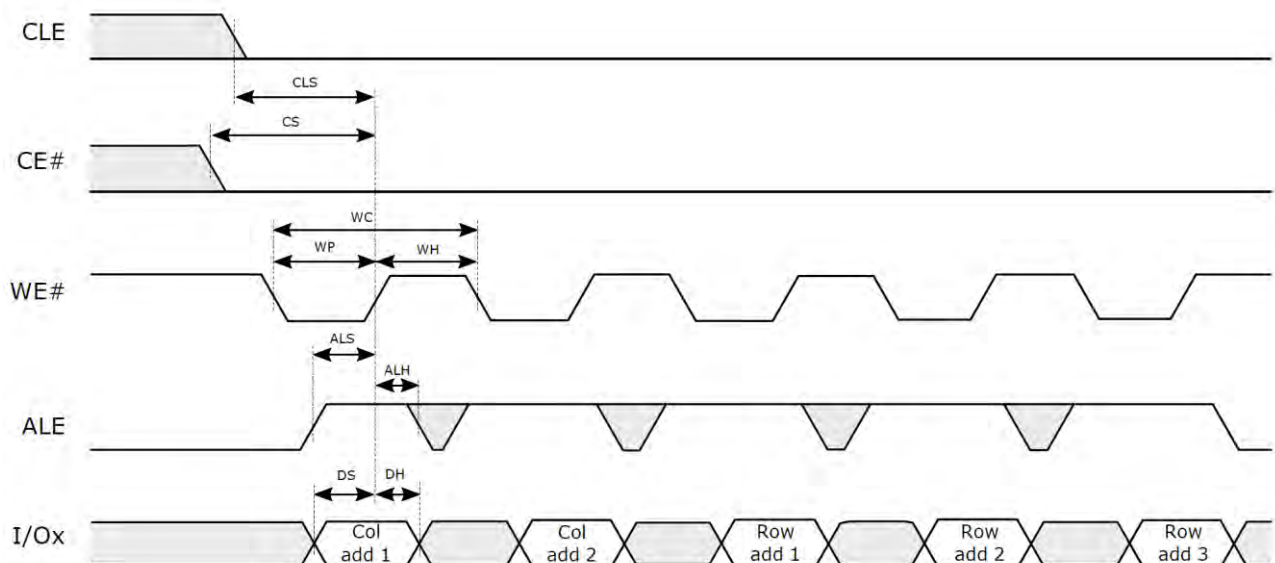
Figure 3-21 NFI ONFI1.0 Address Input Cycle
