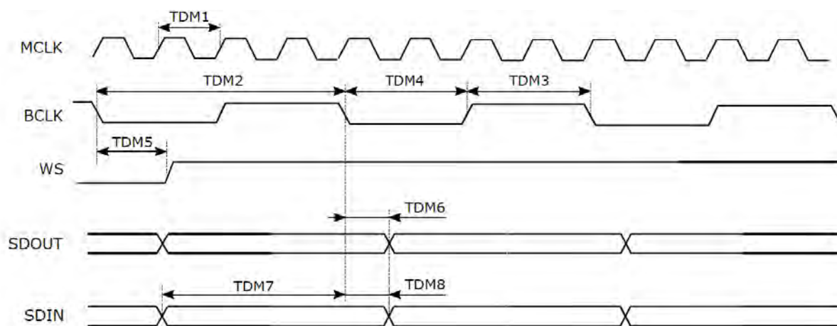
Figure 3-43 TDM Master Mode Timing Diagram
