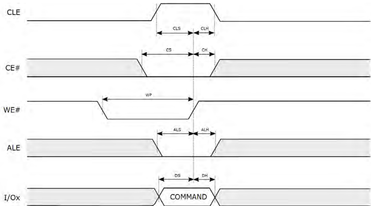
Figure 3-20 NFI ONFI1.0 Command Input Cycle
