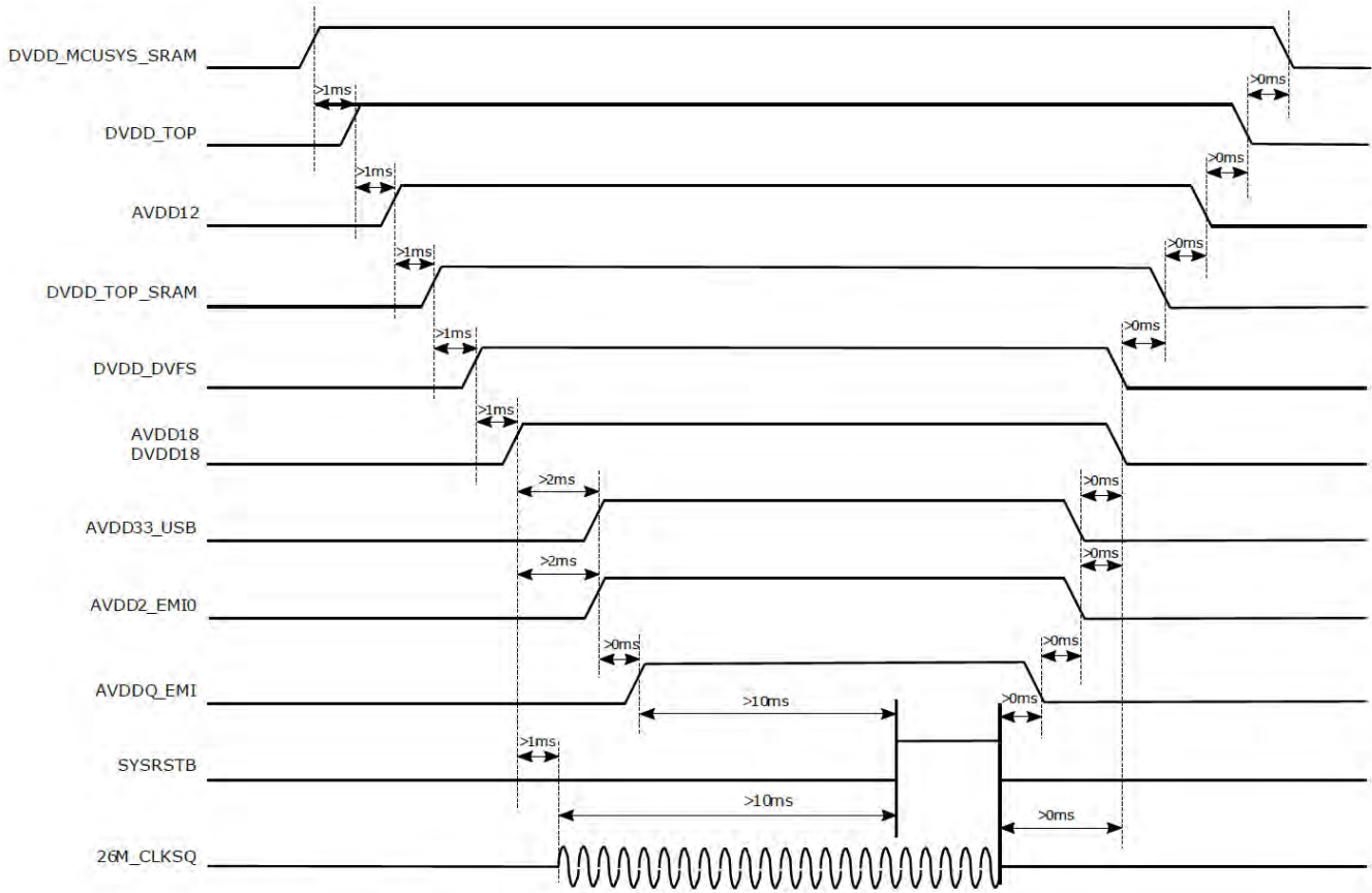
Figure 5-1 Power-on/Power-off Sequence
