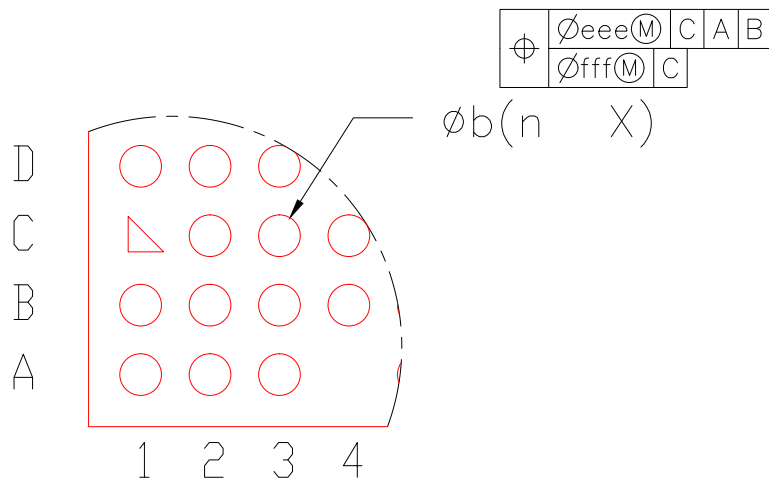
DETAIL : "B"
