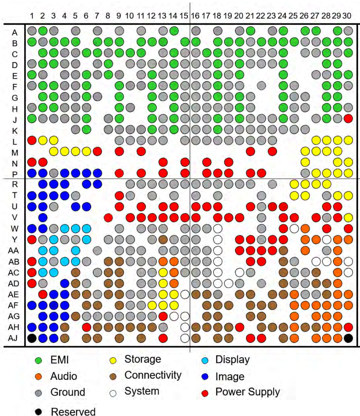
Figure 4-1 Ball Map Diagram
