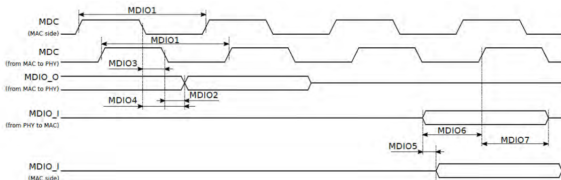
Figure 3-27 ENIC MDIO Timing Diagram
