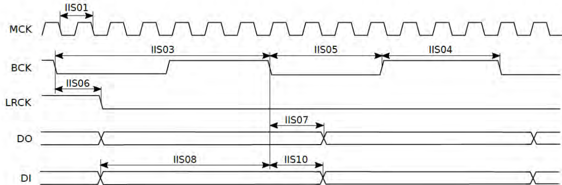
Figure 3-14 I2S Master Mode Timing Diagram
