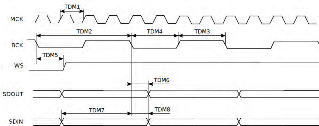
Figure 3-18 TDM Master Mode Timing Diagram
