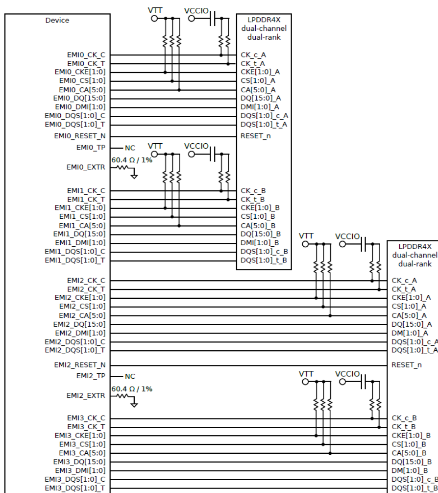
Figure 3-1 LPDDR4X Basic Schematic for 2 \times 2 \times 16 -bit
