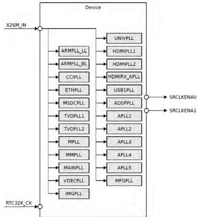
Figure 6-1 Device Clock Diagram
