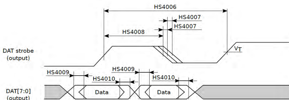
Figure 3-8 MSDC Timing Diagram (HS400 Output mode)
