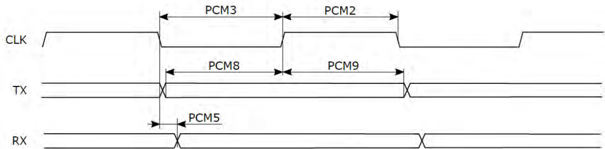
Figure 3-17 PCM Slave Mode Timing Diagram
