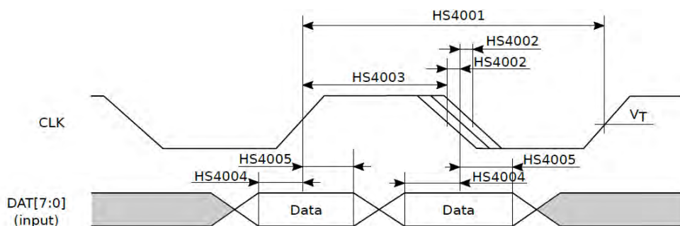
Figure 3-7 MSDC Timing Diagram (HS400 Input mode)
