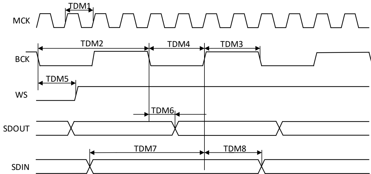
Figure 3-26 TDM master mode timing diagram
