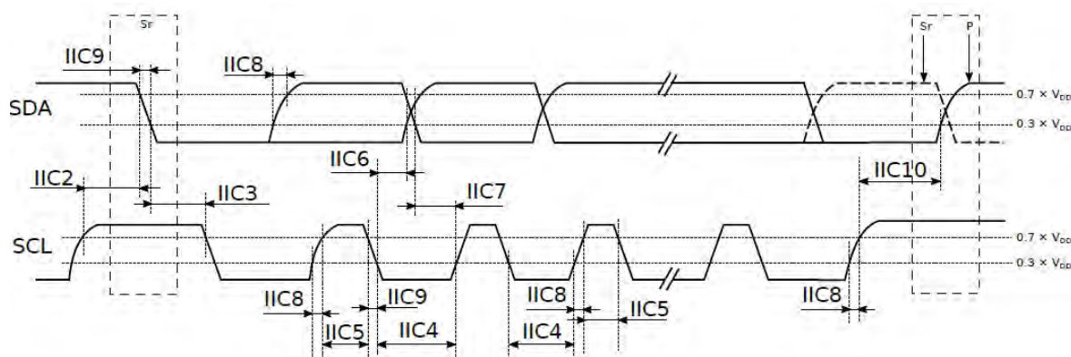
Figure 3-29 I2C timing diagram (HS mode)
