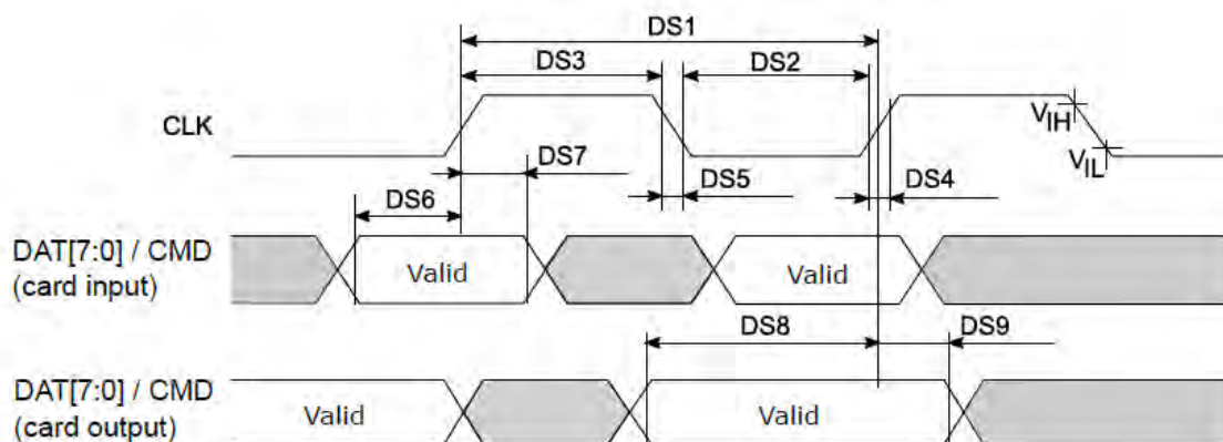
Figure 3-11 MSDC timing diagram (default speed mode)
