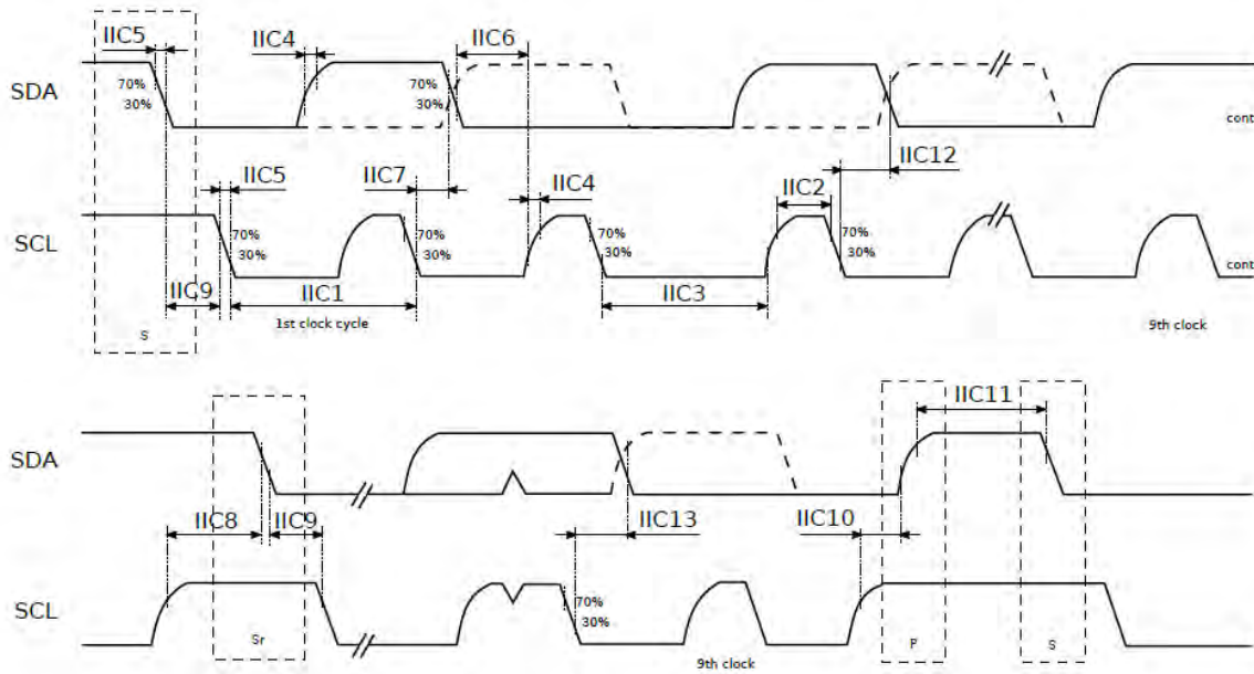
Figure 3-28 I2C timing diagram (SS/FS/FS+ modes)
