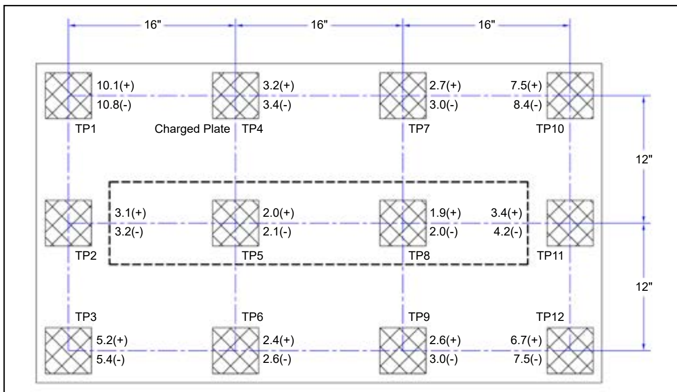
Figure 13. 50681, 50603 Neutralization (Discharge) Times at 220VAC, 50Hz input
