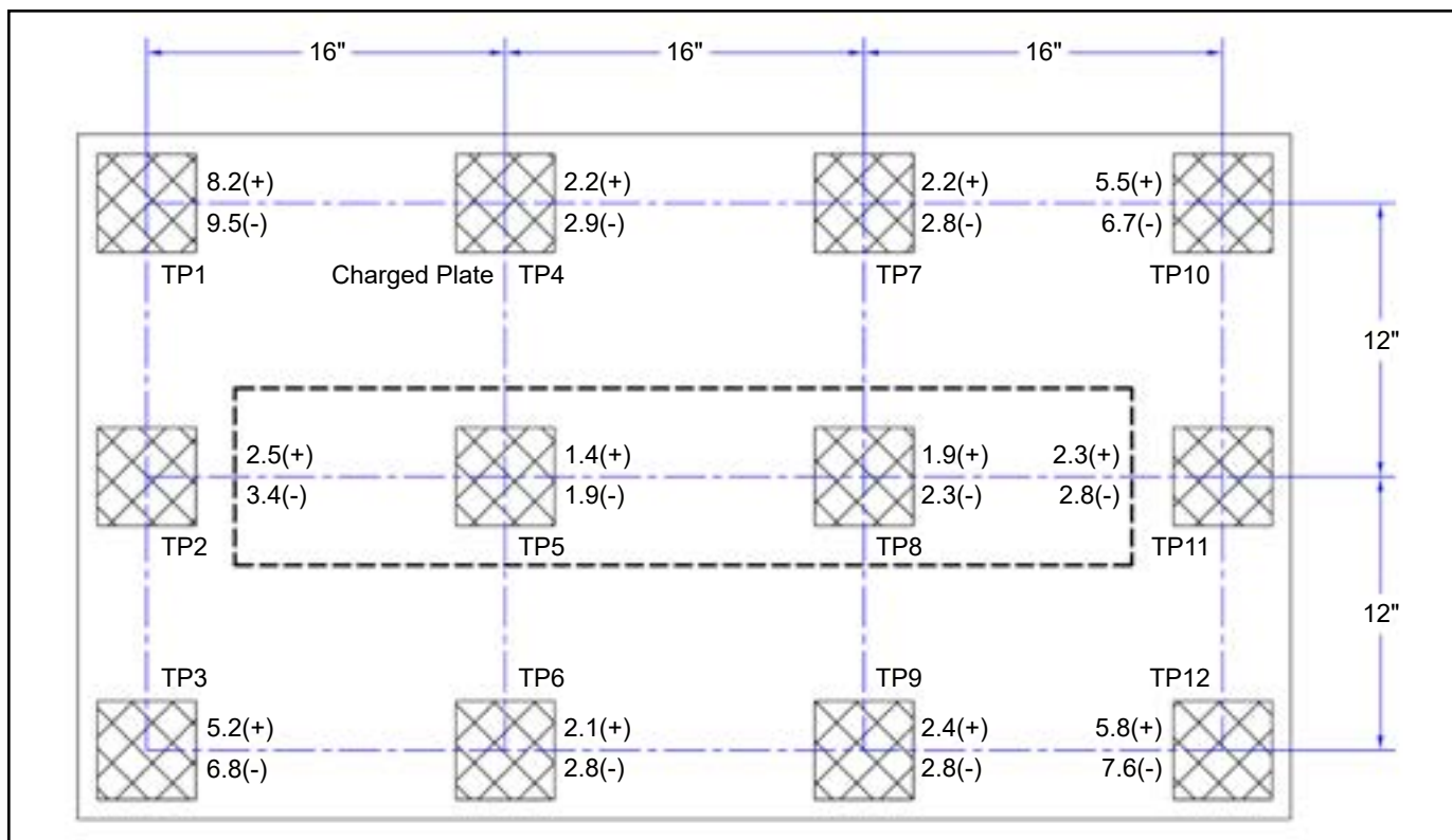
Figure 12. 50681, 50603 Neutralization (Discharge) Times at 120VAC, 60Hz input
