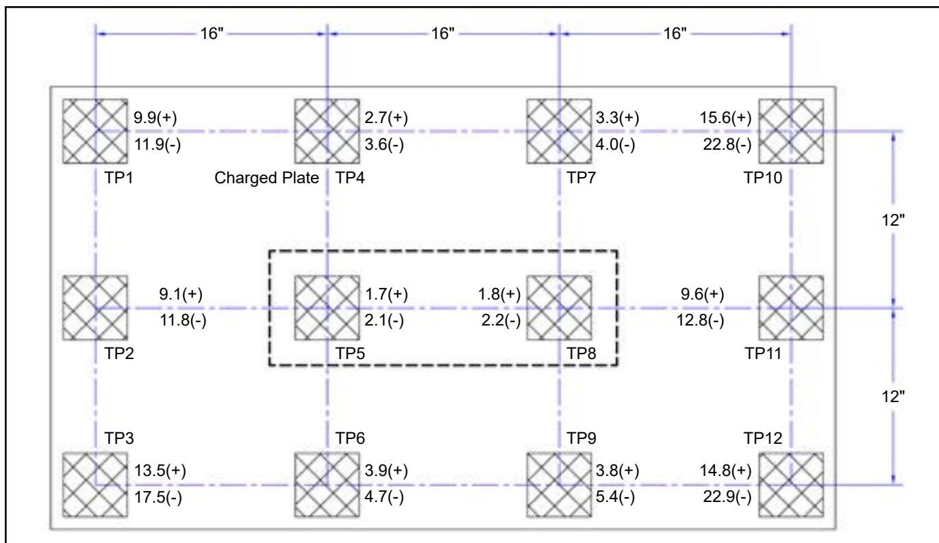
Figure 14. 50682, 50602 Neutralization (Discharge) Times at 100VAC, 50Hz input
