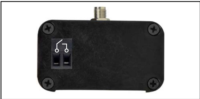
Figure 7. Relay terminal pin-out
