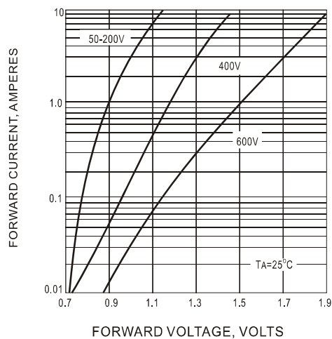
Fig.3 FORWARD CHARACTERISTICS
