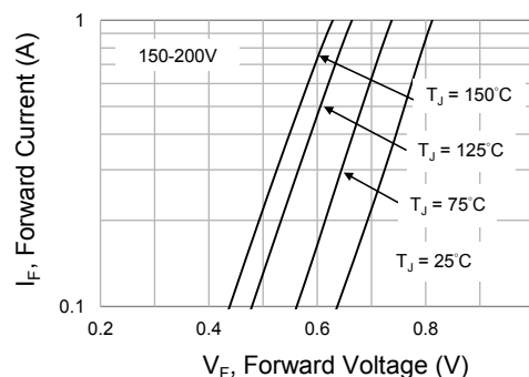
Fig.10 Typical Forward Characteristics
