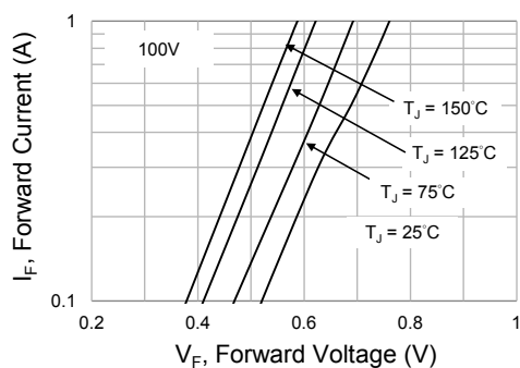
Fig.9 Typical Forward Characteristics
