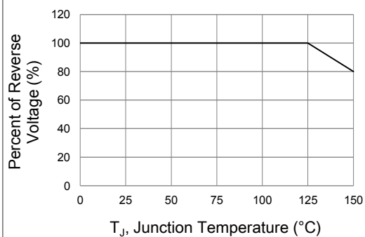
Fig.11 Operating Temperature Derating Curve
