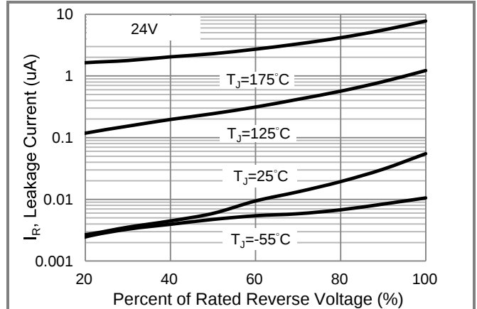
Fig.8 Typical Reverse Characteristics
