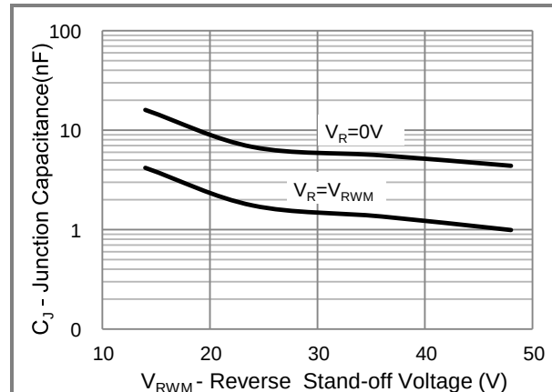
Fig.6 Typical Capacitance
