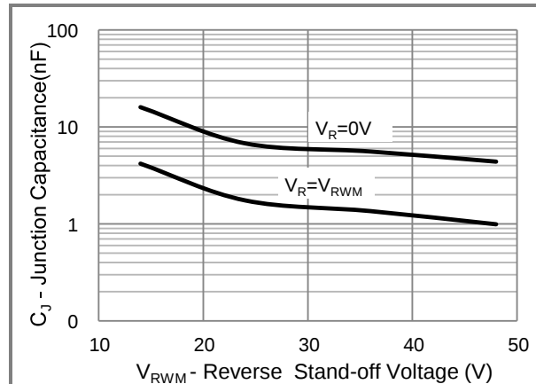
Fig.6 Typical Capacitance
