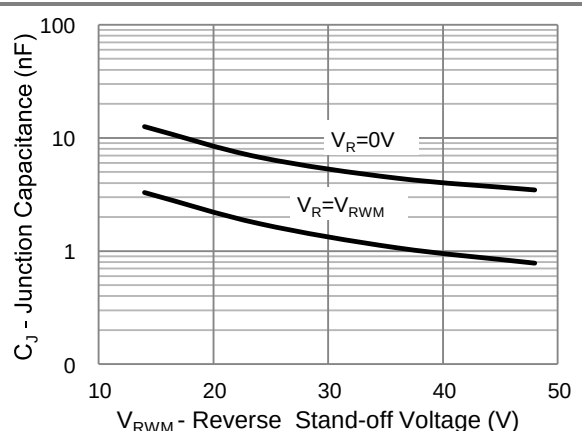
Fig.6 Typical Capacitance
