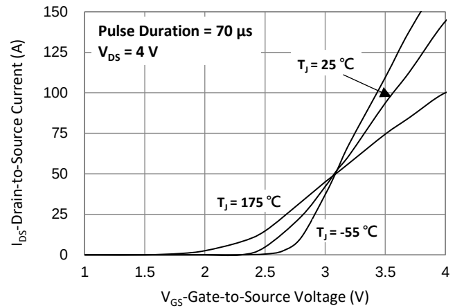
Fig.2 Transfer Characteristics
