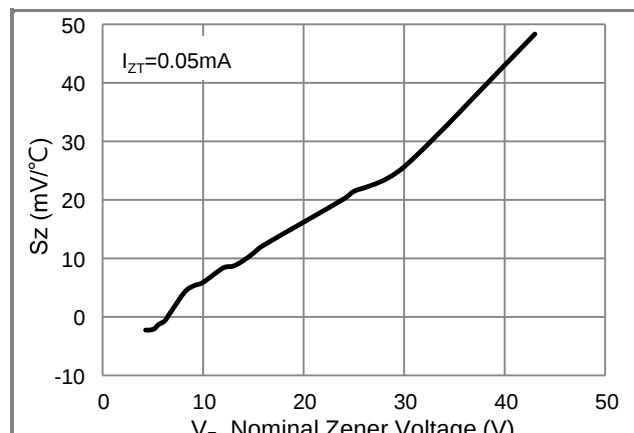
Fig.6 Typical Temperature Coefficient
