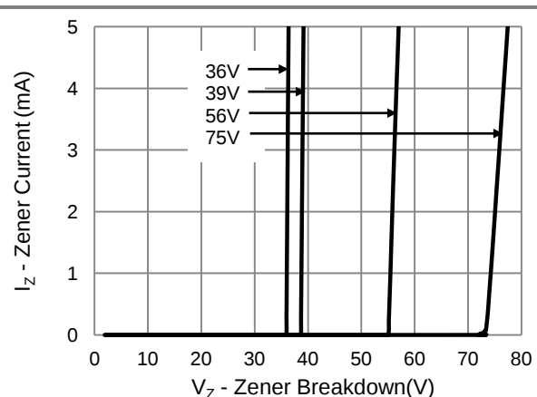
Fig.5 Typical Zener Breakdown
