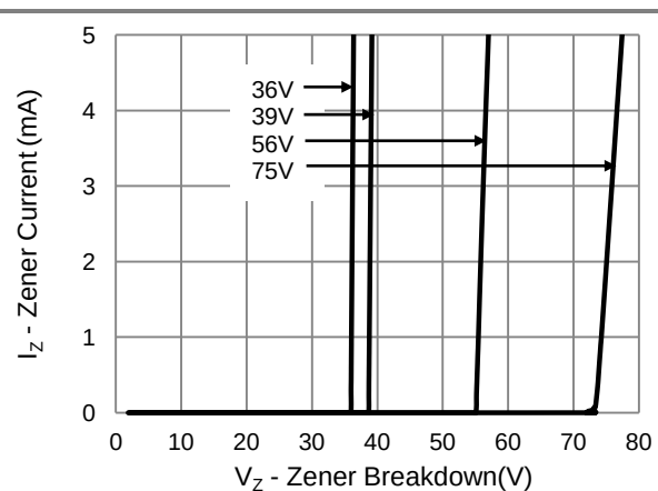
Fig.5 Typical Zener Breakdown
