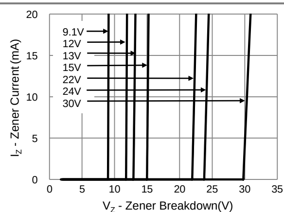
Fig.4 Typical Zener Breakdown
