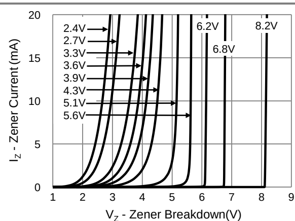
Fig.3 Typical Zener Breakdown
