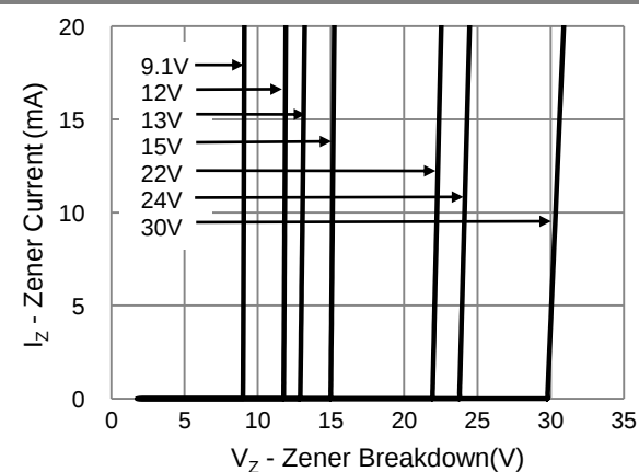
Fig.4 Typical Zener Breakdown
