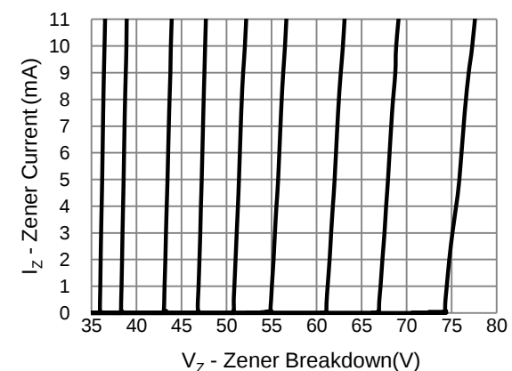
Fig.6 Typical Zener Breakdown
