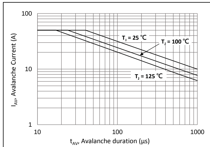
Fig.13 Avalanche Characteristics
