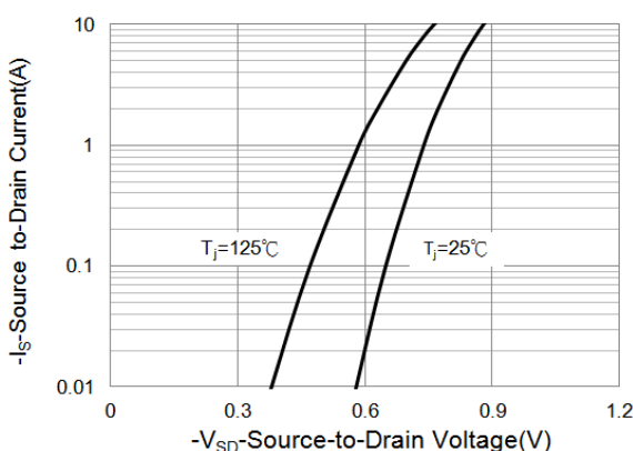
Fig.6 Source-Drain Diode Forward Voltage
