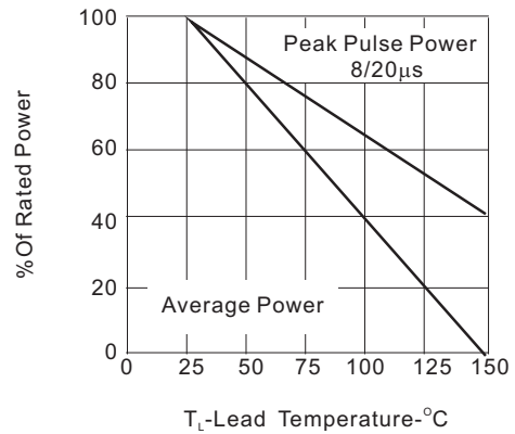
FIG. 2-Power Derating Curve
