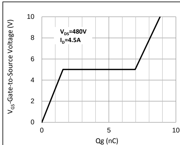
Fig.7 Gate-Charge Characteristics
