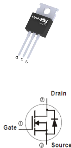
TO-220AB-L
