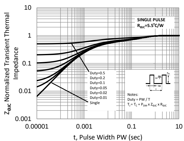
Fig.12 Normalized Transient Thermal Impedance
