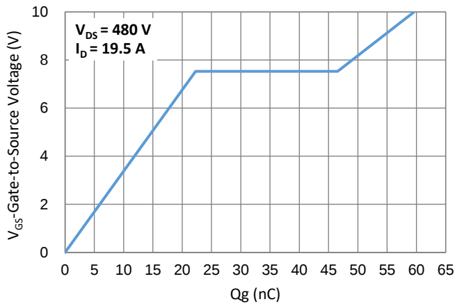
Fig.7 Gate-Charge Characteristics
