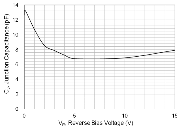
Fig.2 Typical Junction Capacitance(15V)
