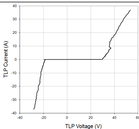
Fig.6 Transmission Line Pulsing (TLP) Measurement
