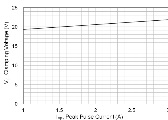
Fig.4 Typical Peak Clamping Voltage(8/20μs)(15V)
