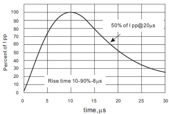
Fig.5 8/20μs Pulse Waveform
