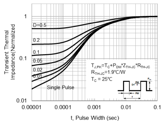
Fig.12 Normalized Transient Thermal Impedance
