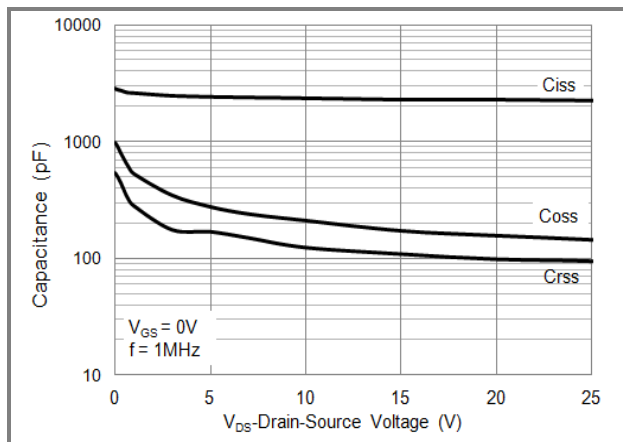
Fig.8 Capacitance vs. Drain-Source Voltage
