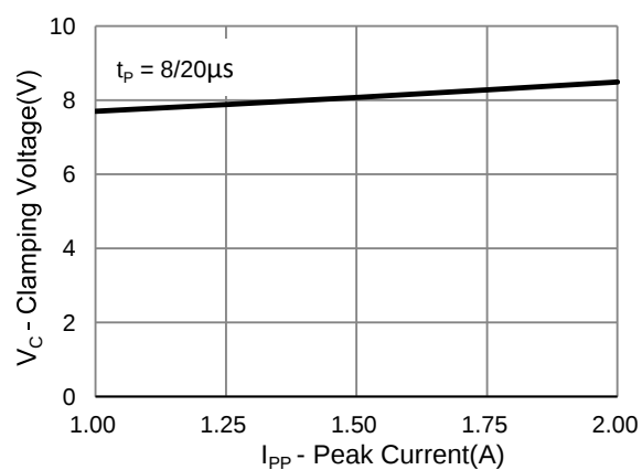
Fig.1 Typical Peak Clamping
