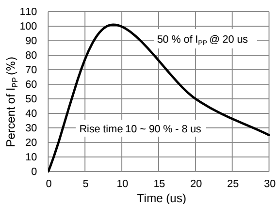
Fig.2 Pulse Waveform
