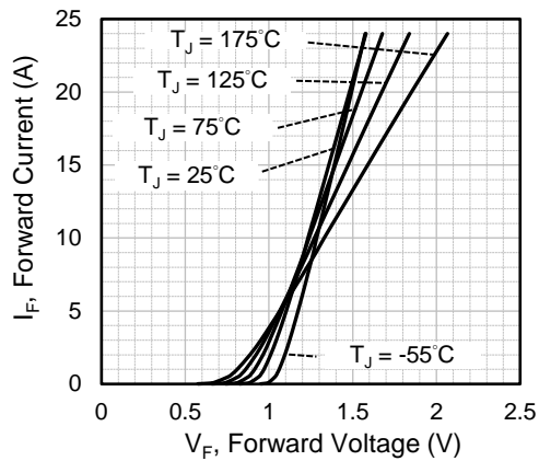
Fig.1 Forward Characteristics
