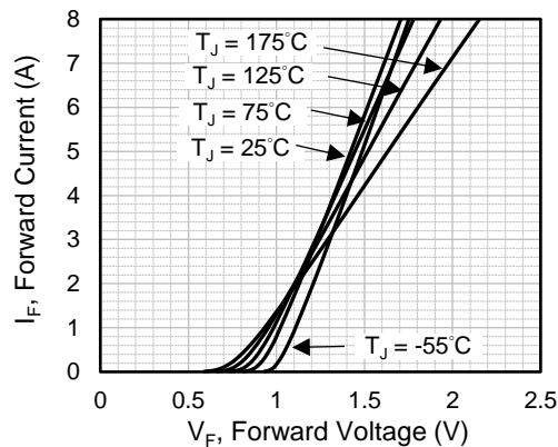
Fig.1 Forward Characteristics
