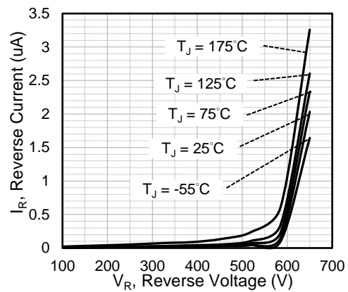
Fig.2 Reverse Characteristics
