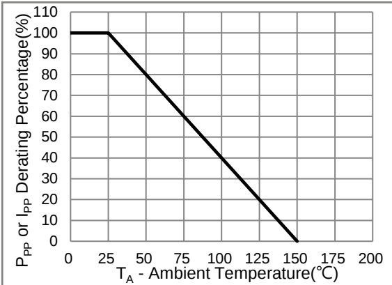
Fig.2 Derating Curve
